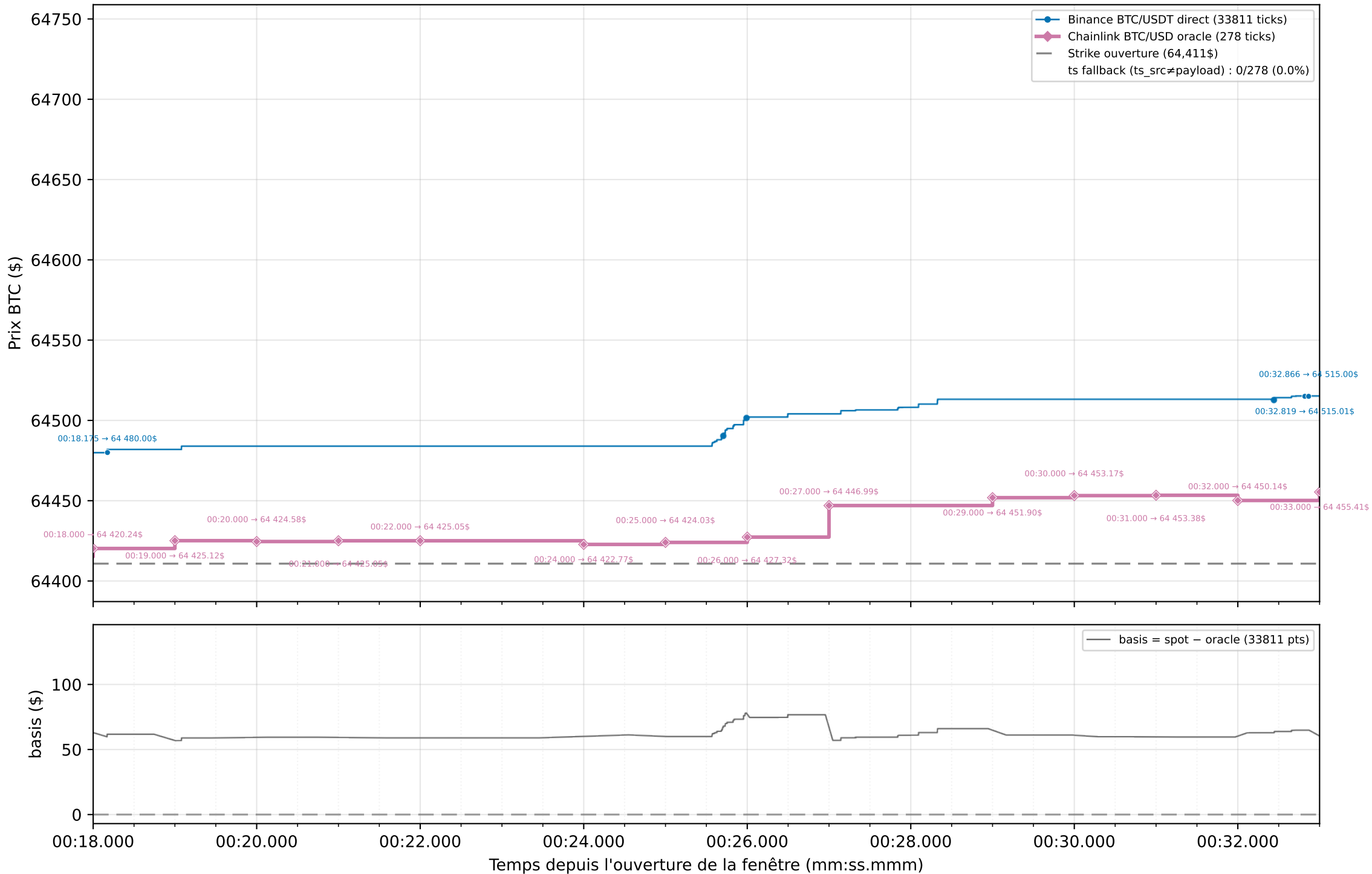
Graphique 2 : Spot Binance (flux direct) vs Oracle Chainlink — strike exact (dernier tick \leq t_0 ) — zoom 15 s [00:18.000 → 00:33.000]
