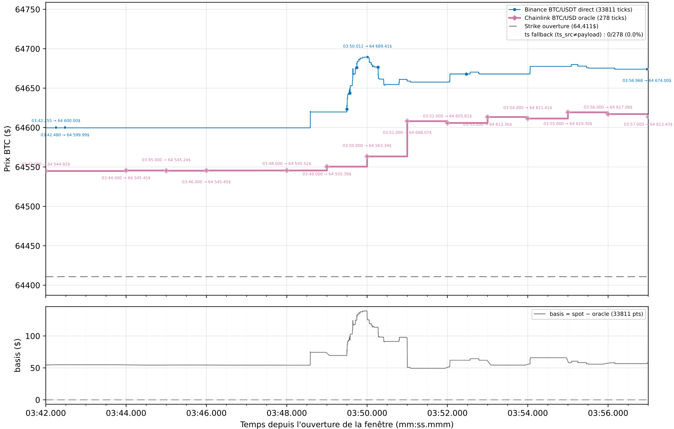
Graphique 2 : Spot Binance (flux direct) vs Oracle Chainlink — strike exact (dernier tick \leq t_0 ) — zoom 15 s [03:42.000 → 03:57.000]
