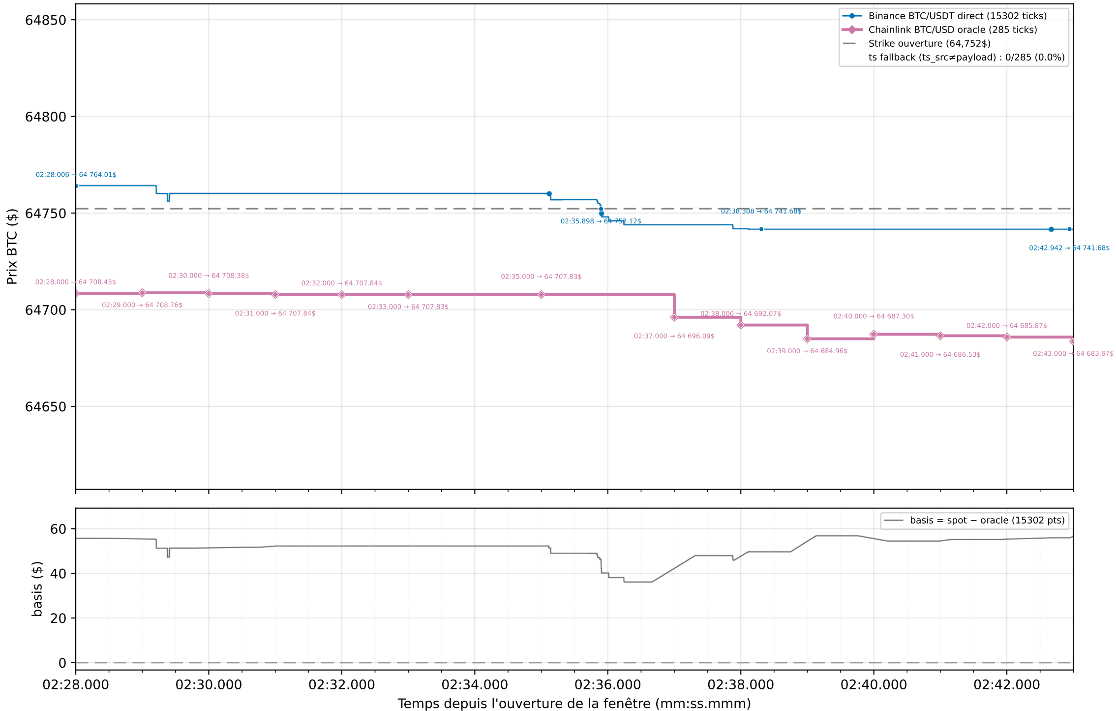
Graphique 2 : Spot Binance (flux direct) vs Oracle Chainlink — strike exact (dernier tick \leq t_0 ) — zoom 15 s [02:28.000 → 02:43.000]
