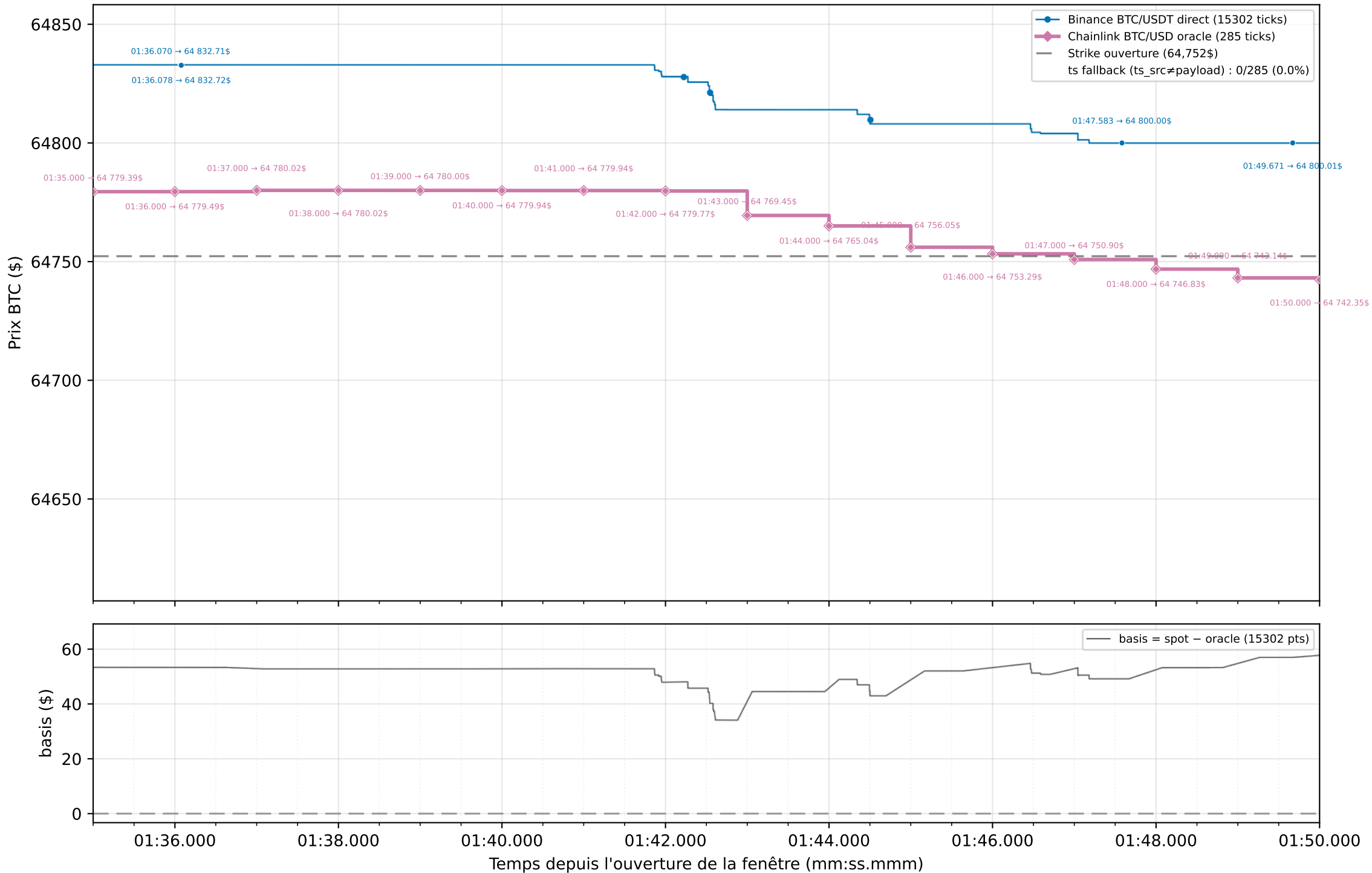
Graphique 2 : Spot Binance (flux direct) vs Oracle Chainlink — strike exact (dernier tick ≤ t0) — zoom 15 s [01:35.000 → 01:50.000]
