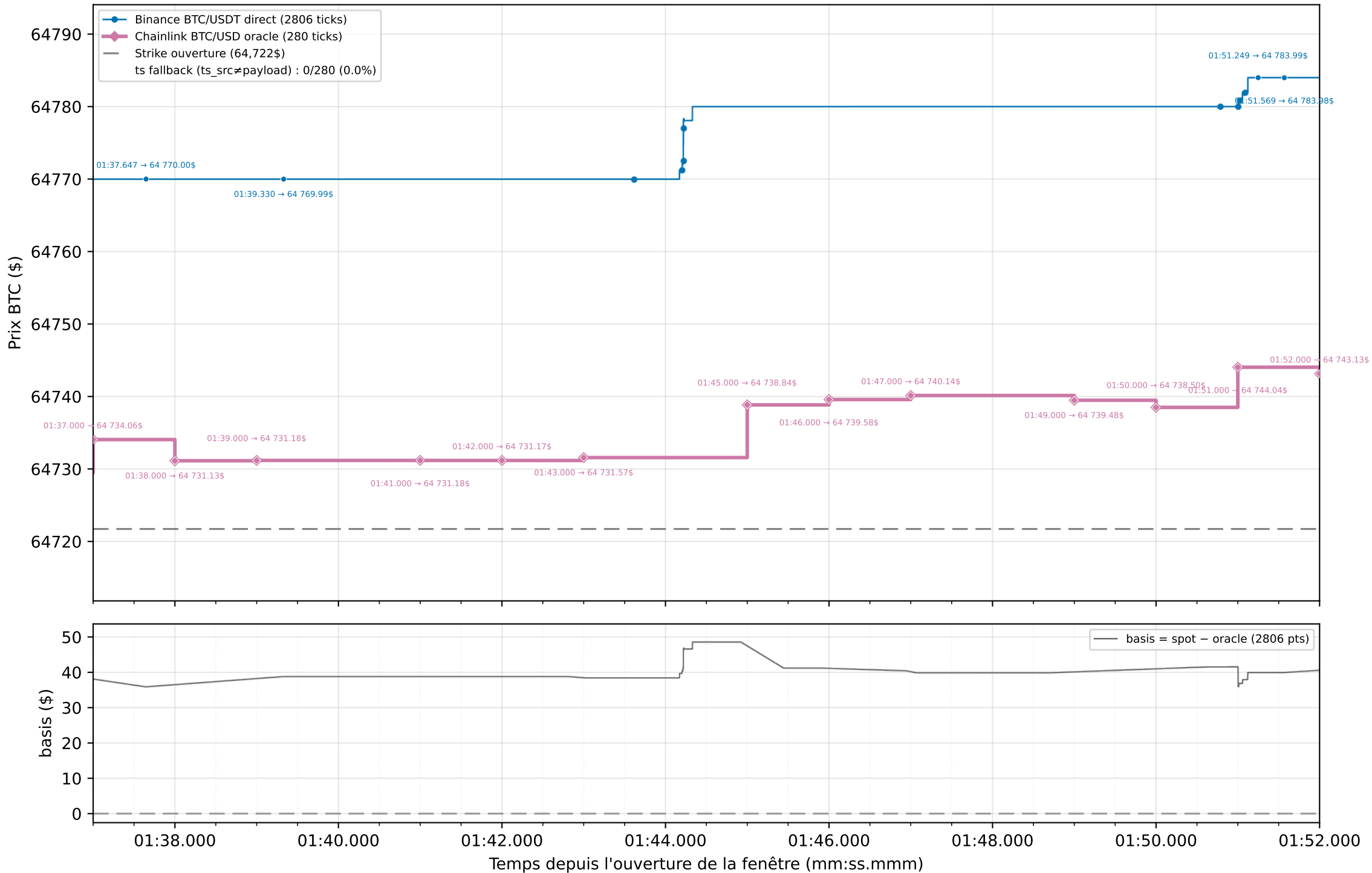
Graphique 2 : Spot Binance (flux direct) vs Oracle Chainlink — strike exact (dernier tick \leq t_0 ) — zoom 15 s [01:37.000 → 01:52.000]
