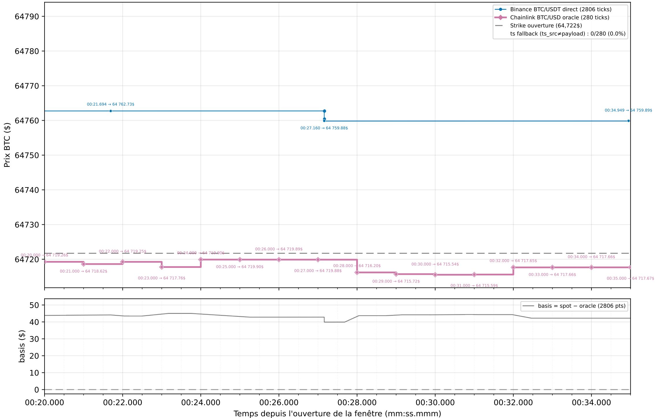
Graphique 2 : Spot Binance (flux direct) vs Oracle Chainlink — strike exact (dernier tick \leq t_0 ) — zoom 15 s [00:20.000 → 00:35.000]
