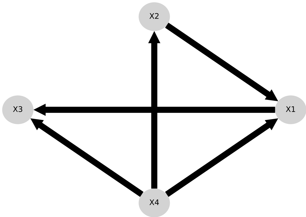
DAG Causal Graph
