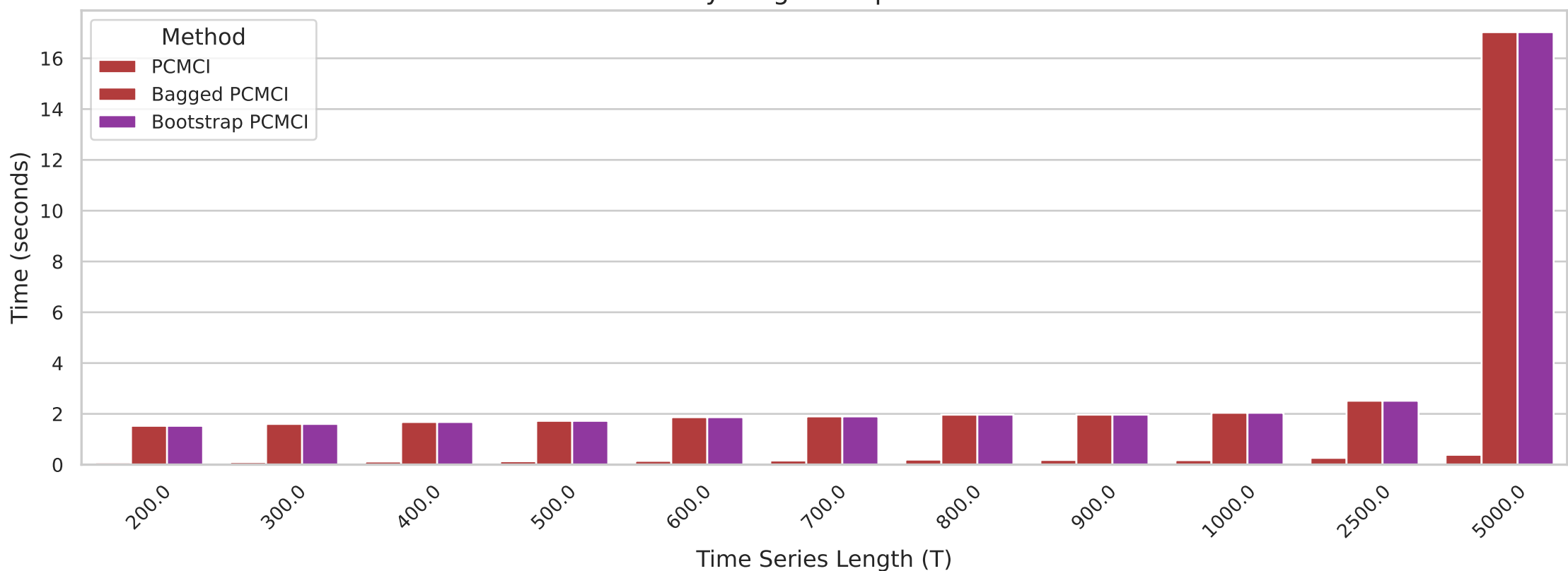
Effect Estimation Stage Computation Time
