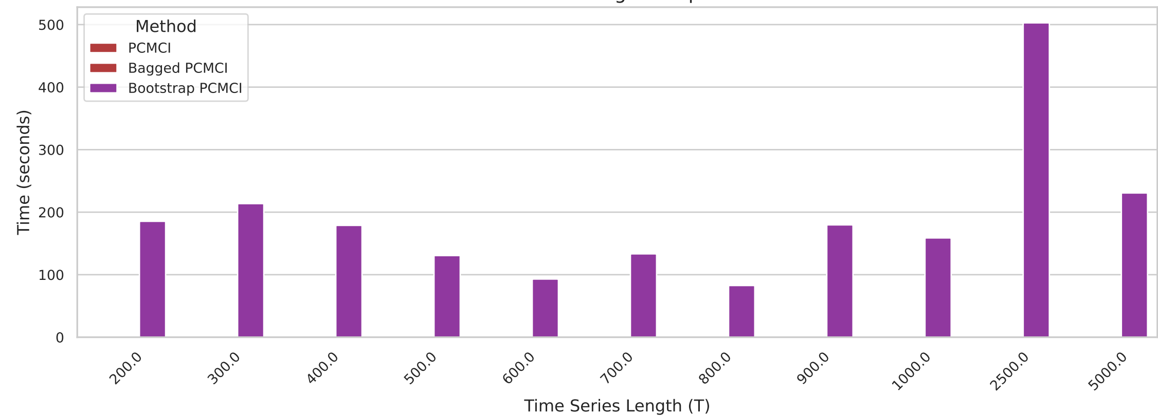
Effect Estimation Stage Computation Time
