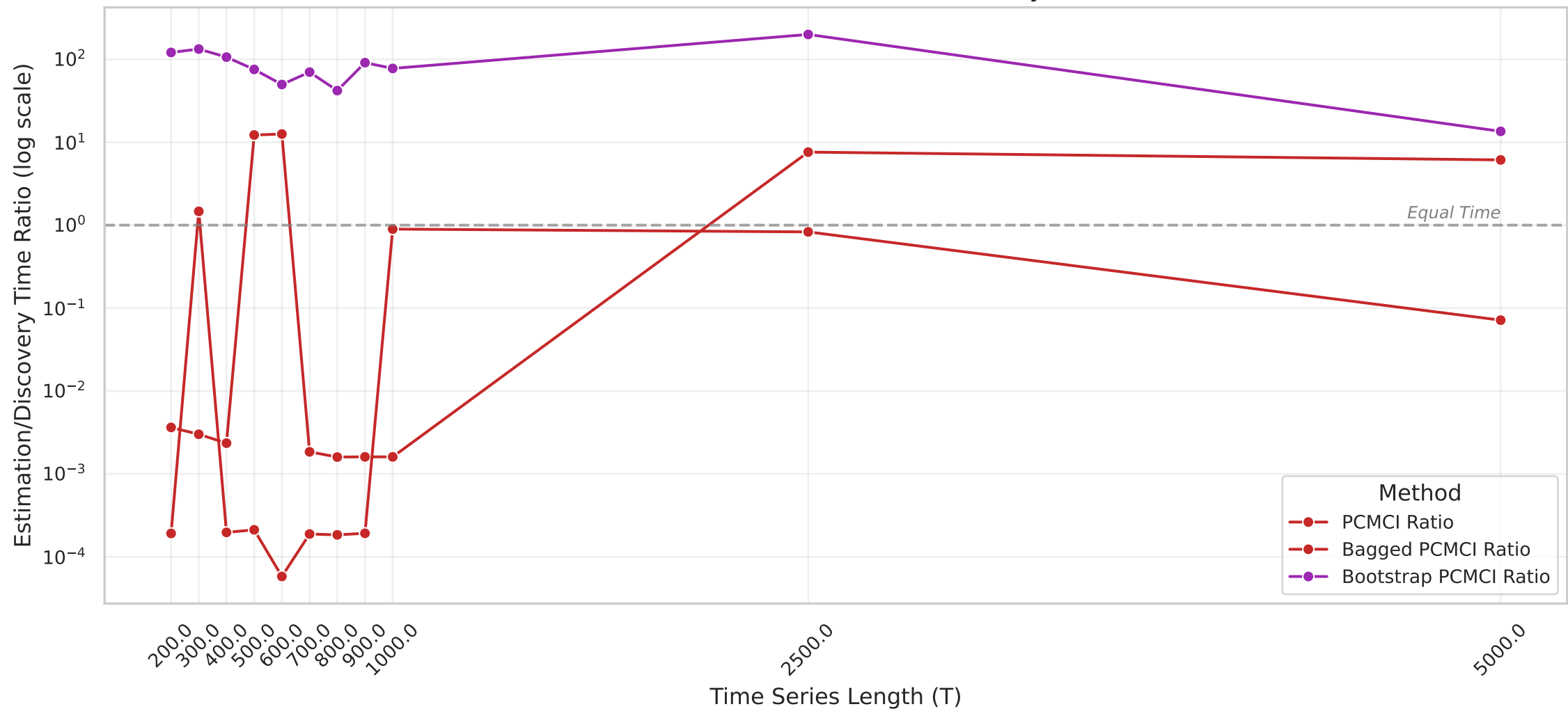
Ratio of Estimation Time to Discovery Time
