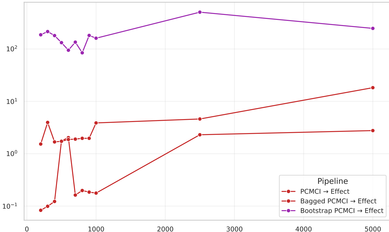
Time Series Length (T), log scale
