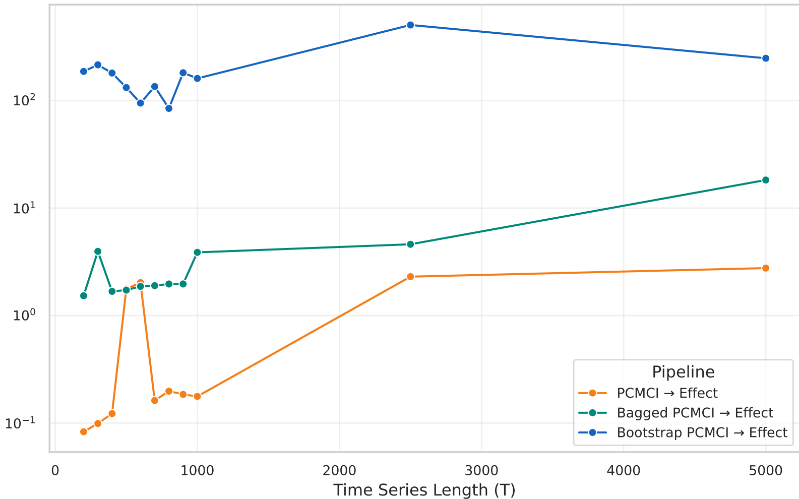
Computation Time (seconds, log scale)
