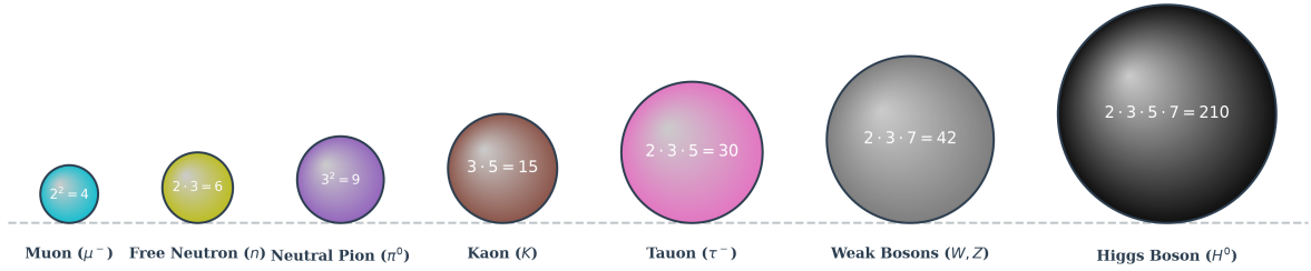
Figure 5: Geometric representation of the unstable and composite particle states ( \mu^- , free neutron, \pi^0 , Kaon, \tau^- , weak bosons, and Higgs boson) ordered by their resonance factor and aligned flush to a common white baseline. The progression in sphere size visualizes the increasing topological complexity and modular composition on the P_4 = 210 vacuum grid.
