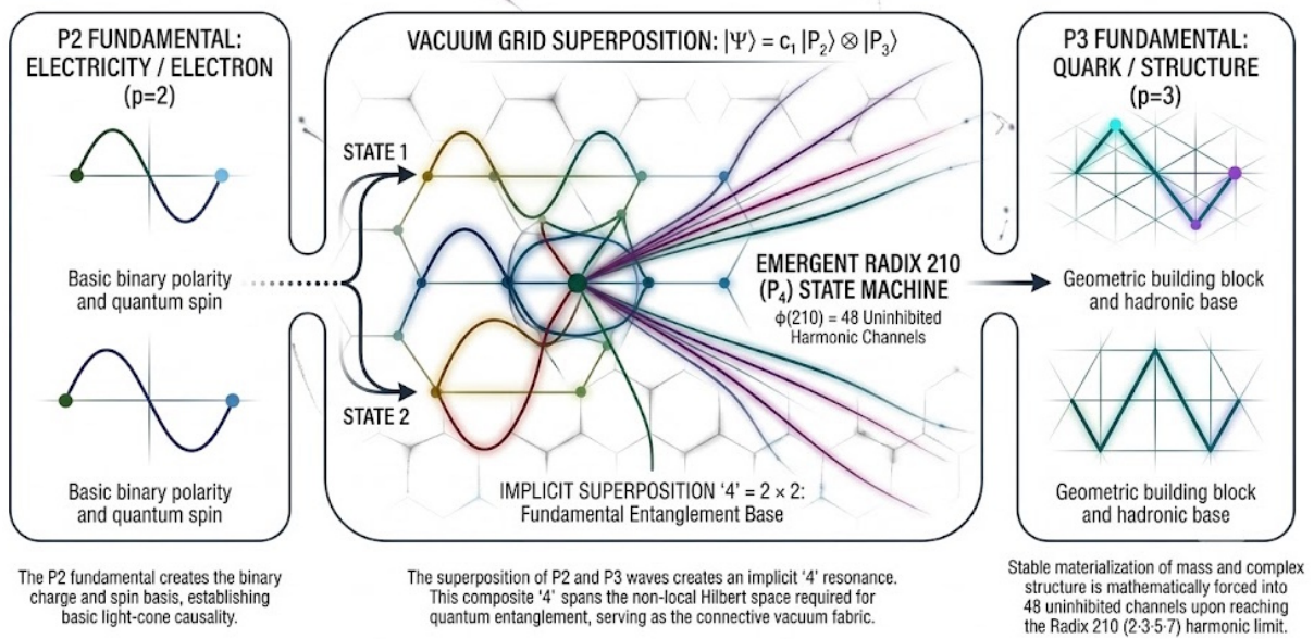
Figure 6: Topological mapping of the vacuum grid superposition and the emergent Radix-210 state machine. The fundamental binary charge/spin wave ( p = 2 ) and the geometric structural wave ( p = 3 ) interfere on the hexagonal vacuum lattice. Their intersection forms an implicit 4 = 2 \times 2 superposition, spanning the 4-dimensional Hilbert space required for non-local quantum entanglement. This entangled baseline channels the discrete prime nodes ( P_4 ) into a coherent, non-damped harmonic framework capped at the \phi(210) = 48 saturation limit.
