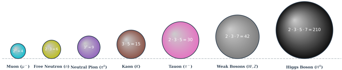
Figure 5: Geometric representation of the unstable and composite particle states ( \mu^- , free neutron, \pi^0 , Kaon, \tau^- , weak bosons, and Higgs boson) ordered by their resonance factor and aligned flush to a common white baseline. The progression in sphere size visualizes the increasing topological complexity and modular composition on the P_4 = 210 vacuum grid.
