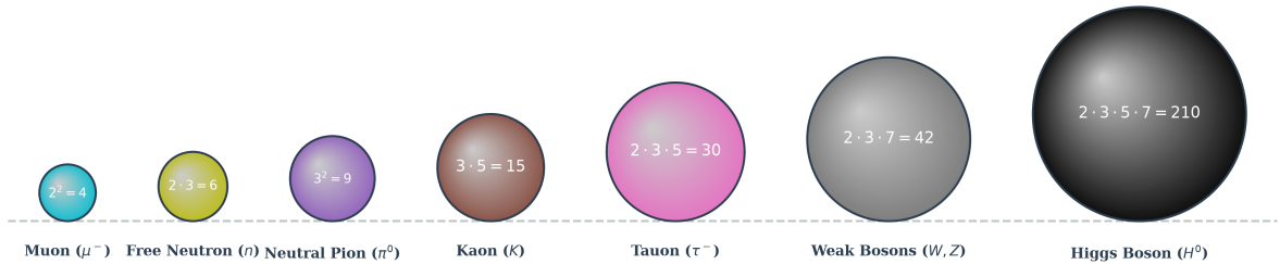
Figure 4: Geometric representation of the unstable and composite particle states ( \mu^- , free neutron, \pi^0 , Kaon, \tau^- , weak bosons, and Higgs boson) ordered by their resonance factor and aligned flush to a common white baseline. The progression in sphere size visualizes the increasing topological complexity and modular composition on the P_4 = 210 vacuum grid.
