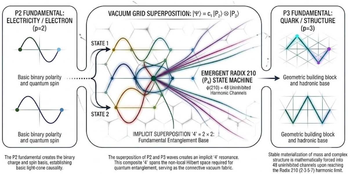
Figure 5: Topological mapping of the vacuum grid superposition and the emergent Radix-210 state machine. The fundamental binary charge/spin wave ( p = 2 ) and the geometric structural wave ( p = 3 ) interfere on the hexagonal vacuum lattice. Their intersection forms an implicit 4 = 2 \times 2 superposition, spanning the 4-dimensional Hilbert space required for non-local quantum entanglement. This entangled baseline channels the discrete prime nodes ( P_4 ) into a coherent, non-damped harmonic framework capped at the \phi(210) = 48 saturation limit.
