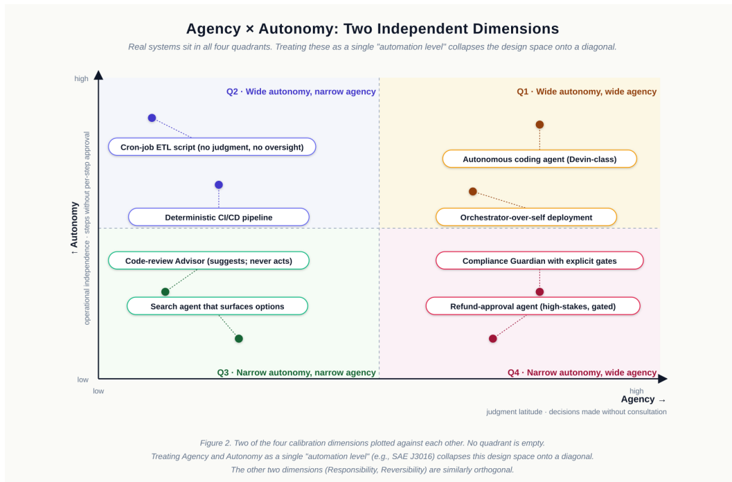
Figure 2: Figure 2. Two of the four calibration dimensions plotted against each other. Each quadrant has real deployments; no quadrant is empty. The other two dimensions (Responsibility, Reversibility) are similarly orthogonal. Treating Agency and Autonomy as a single “automation level” — as SAE J3016 does for driving (SAE International 2021) — collapses this design space onto a diagonal.
