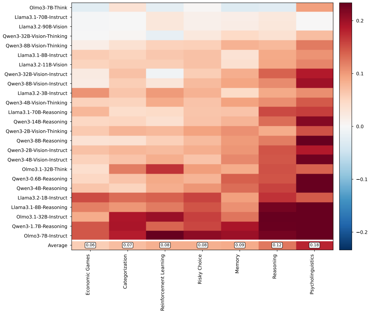
Post-training misalignment
