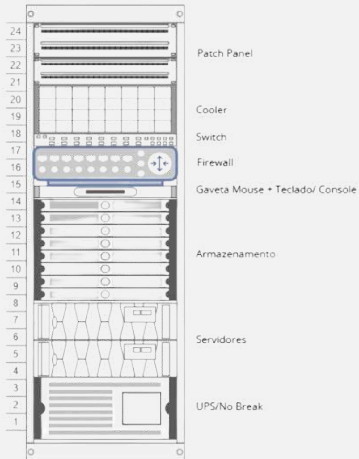
Rack 24U
