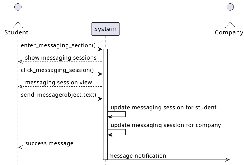
Figure 3.32: Student message providing Sequence Diagram
