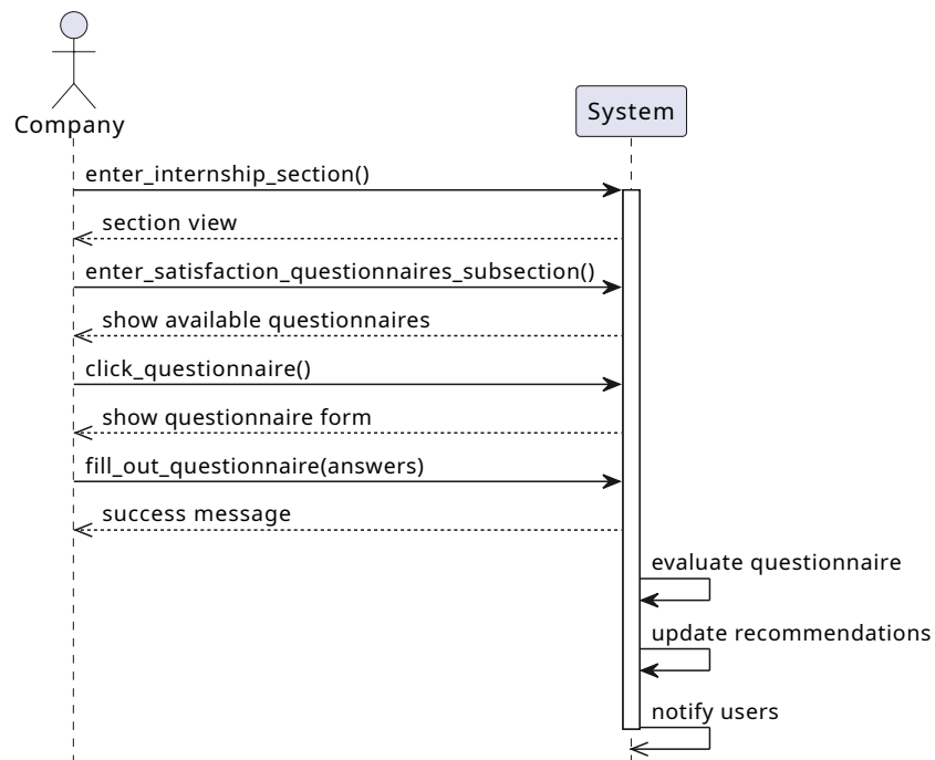
Figure 3.31: Company satisfaction questionnaire compilation Sequence Diagram
