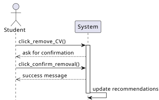
Figure 3.19: CV removal Sequence Diagram
