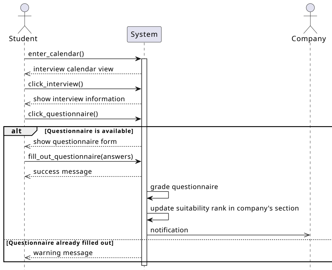
Figure 3.27: Selection process questionnaire compilation Sequence Diagram
