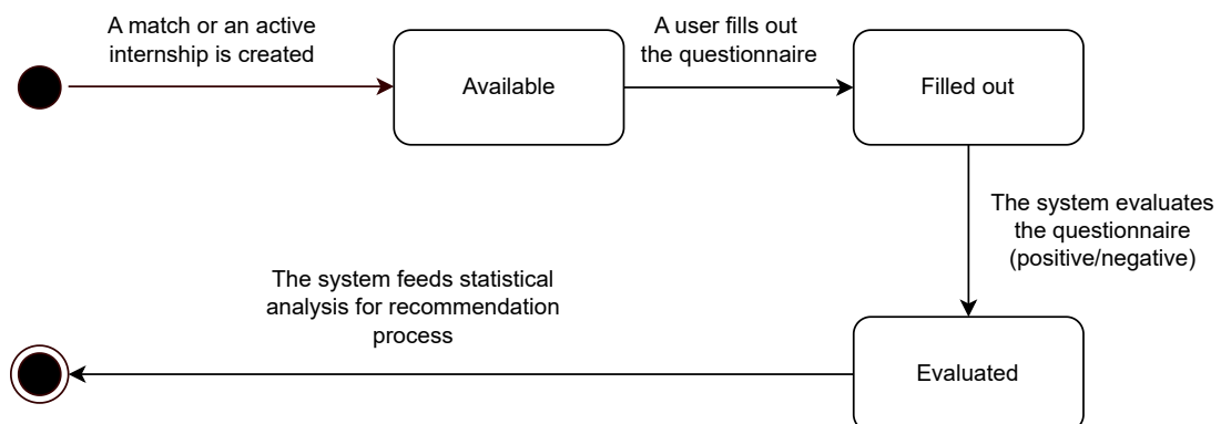
Figure 2.4: Satisfaction questionnaire state diagram
