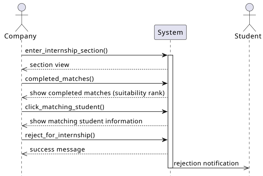
Figure 3.29: Student rejection Sequence Diagram
