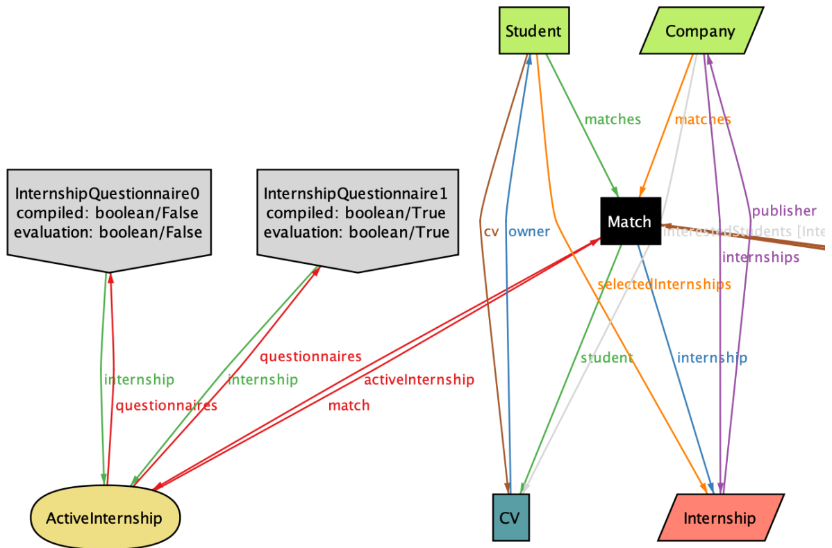
Figure 4.2: World example: active internship
