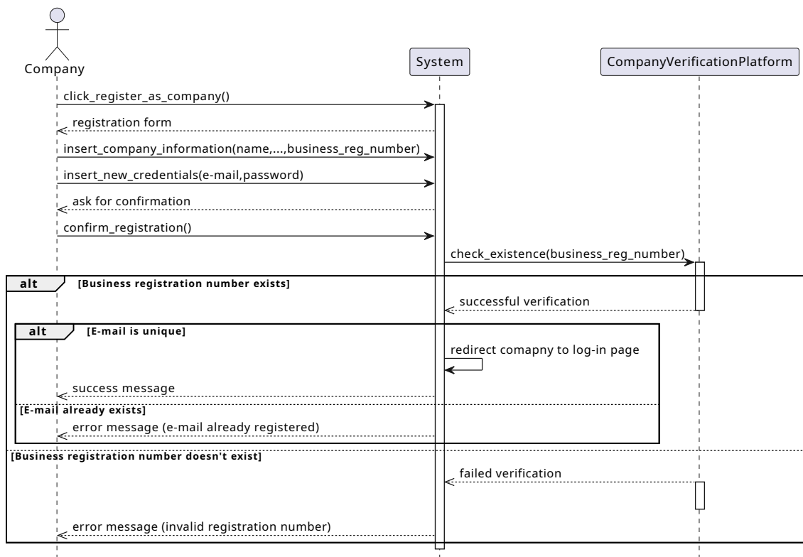
Figure 3.16: Company registration Sequence Diagram
