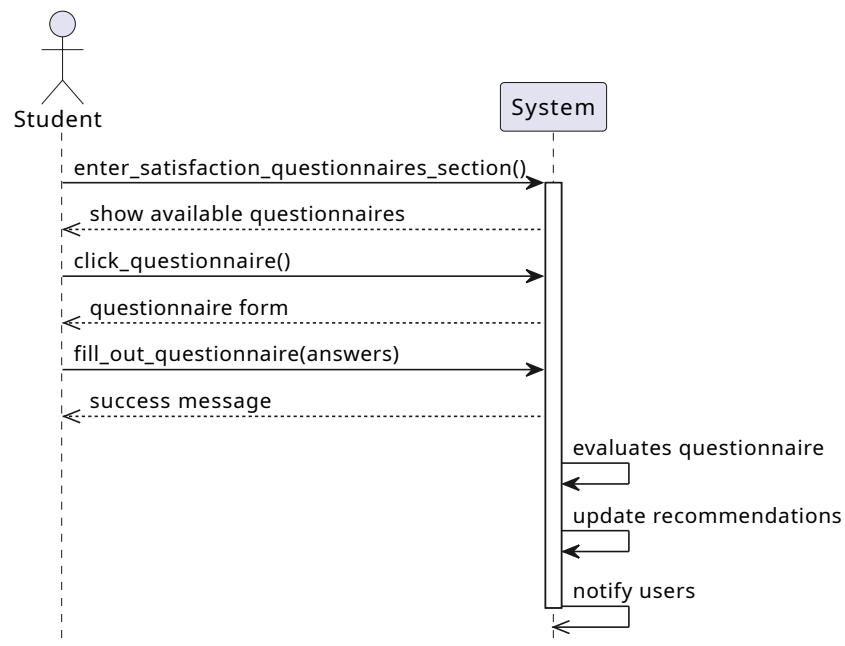
Figure 3.30: Student satisfaction questionnaire compilation Sequence Diagram
