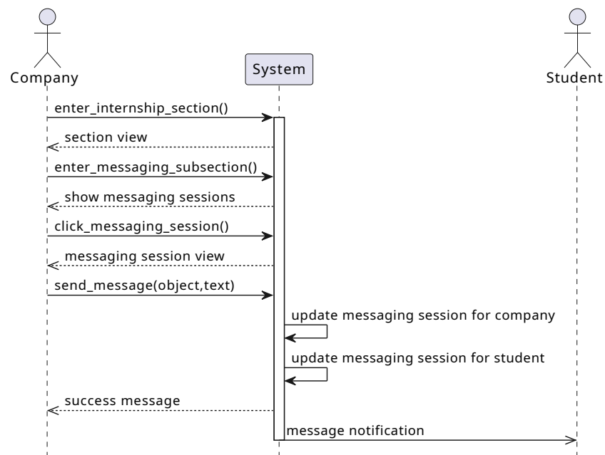
Figure 3.33: Company message providing Sequence Diagram
