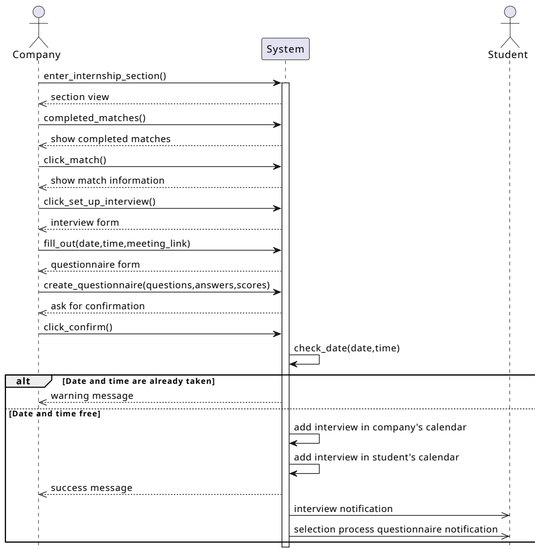
Figure 3.26: Interview set up Sequence Diagram
