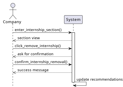
Figure 3.21: Internship removal Sequence Diagram
