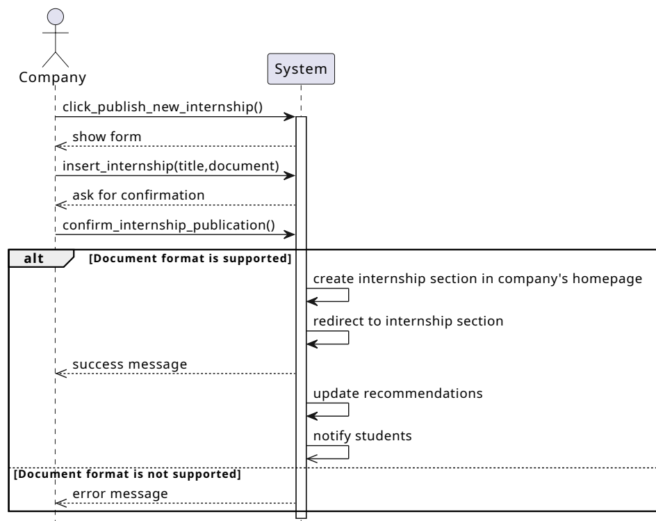
Figure 3.20: Internship publication Sequence Diagram
