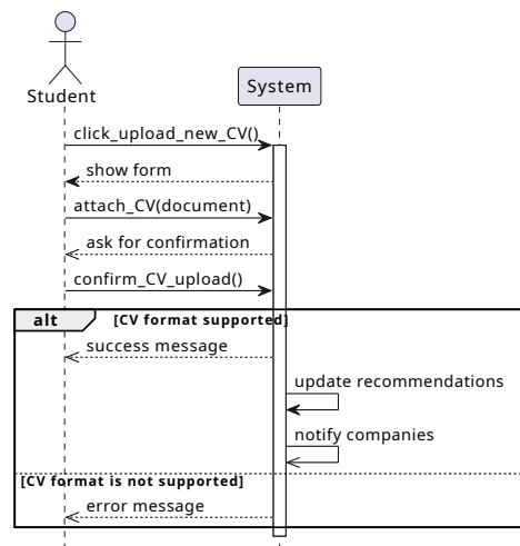
Figure 3.18: CV upload Sequence Diagram
