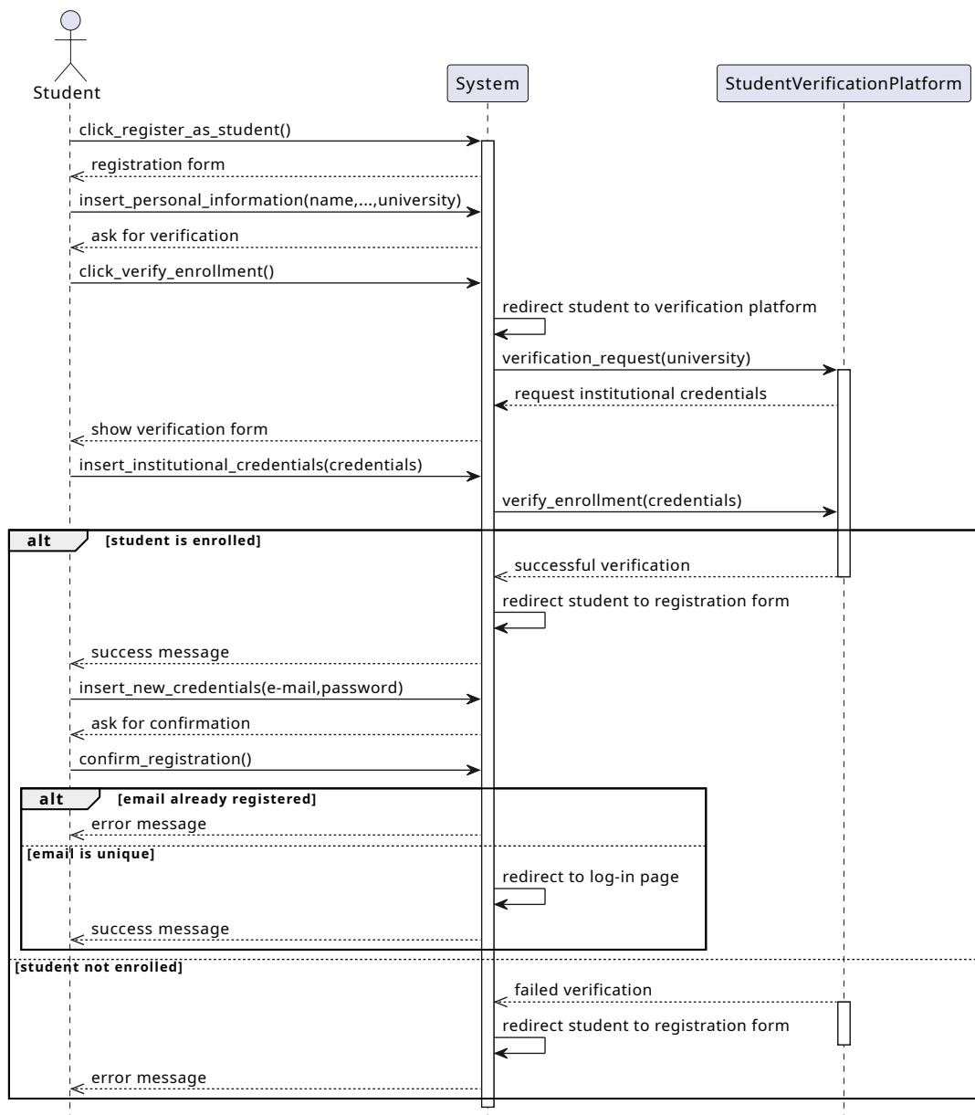
Figure 3.15: Student registration Sequence Diagram
