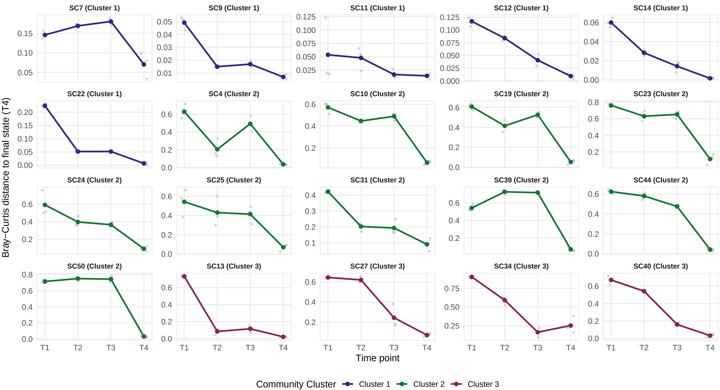
Supplementary Figure 2B: Stabilization toward final community composition
