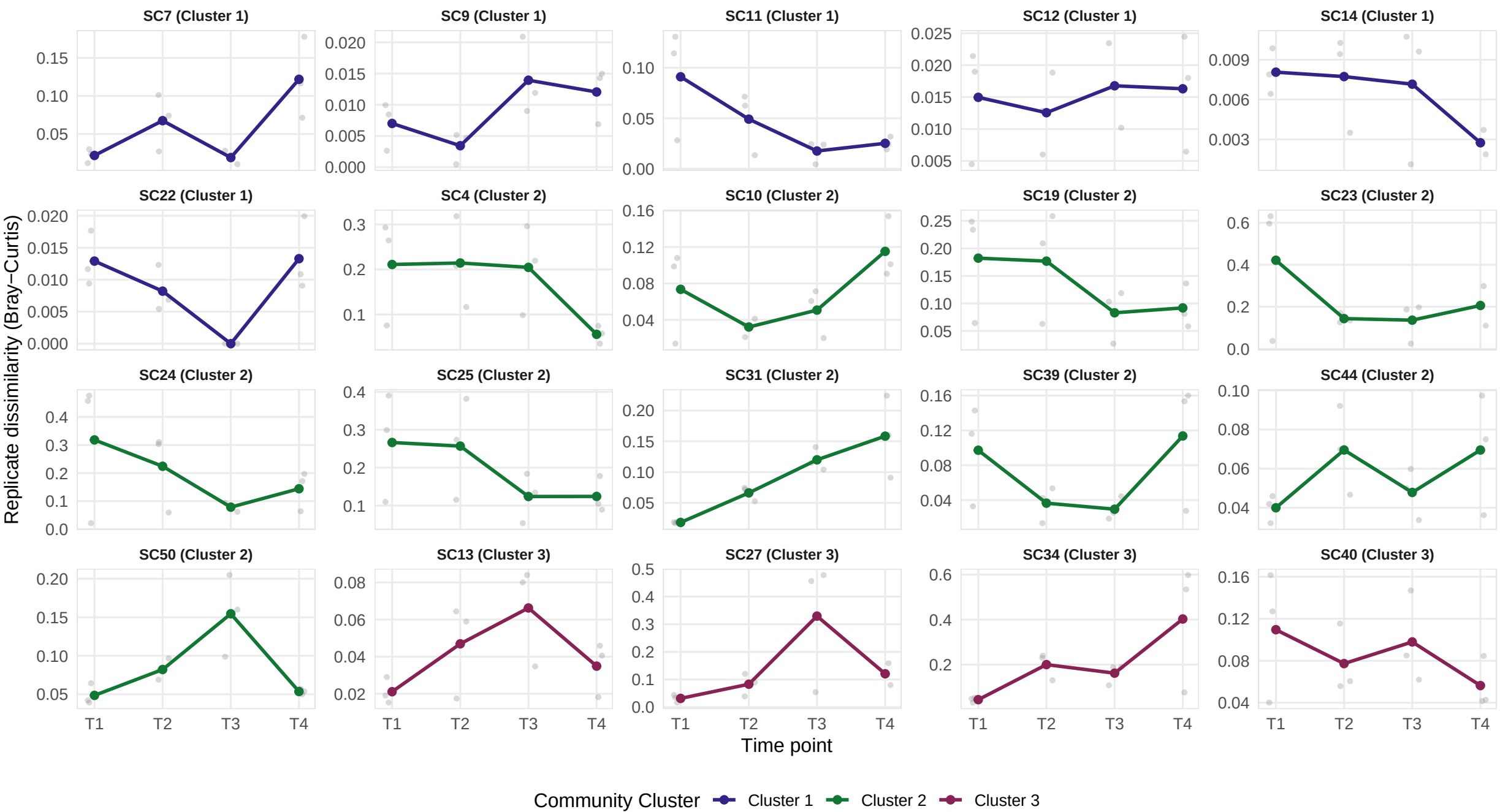
Supplementary Figure 2A: Replicate dissimilarity per SynCom
