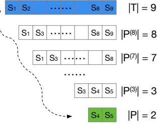
Figure 2: Weak Monotonicity.
