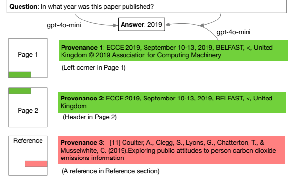
Figure 6: Top-k Provenance.
