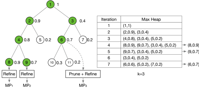
Figure 7: Top-k Provenance.
