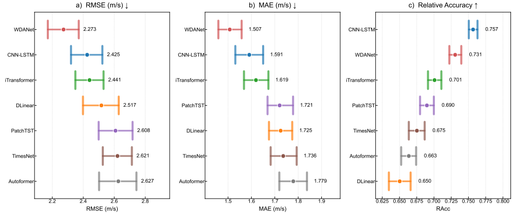
Fig. 2 95% confidence intervals of model performance obtained from typhoon-event block bootstrap. a is RMSE result. b is MAE result. c is RAcc result. The markers represent the mean values of each metric, and the error bars indicate the 95% confidence intervals.
