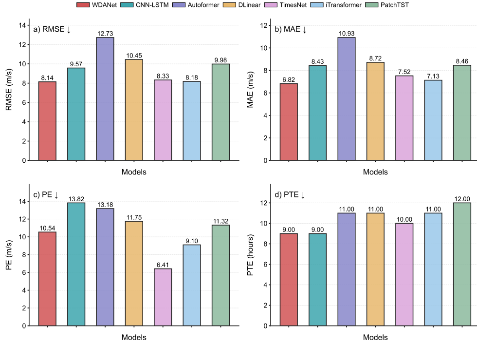
Fig. 5 Forecasting performance of different models during the most intense 24-h gust period of Typhoon Yagi. Performance comparison of different forecasting models during the most intense 24-h gust period of Typhoon Yagi. The selected period represents the consecutive 24 hours with the highest average gust intensity, covering the most challenging extreme wind conditions. The evaluation includes a RMSE, b MAE, c peak error (PE), and d peak time error (PTE). Lower values indicate better performance.
