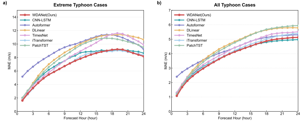
Fig. 3 Performance comparison of multi-step wind gust forecasting under different typhoon scenarios. a MAE under typhoon conditions with maximum wind gusts ranging from 28.52 m/s to 46.85 m/s. b MAE under typhoon conditions with maximum wind gusts exceeding 15 m/s. The horizontal axis denotes the forecast horizon, and the vertical axis represents the error.
