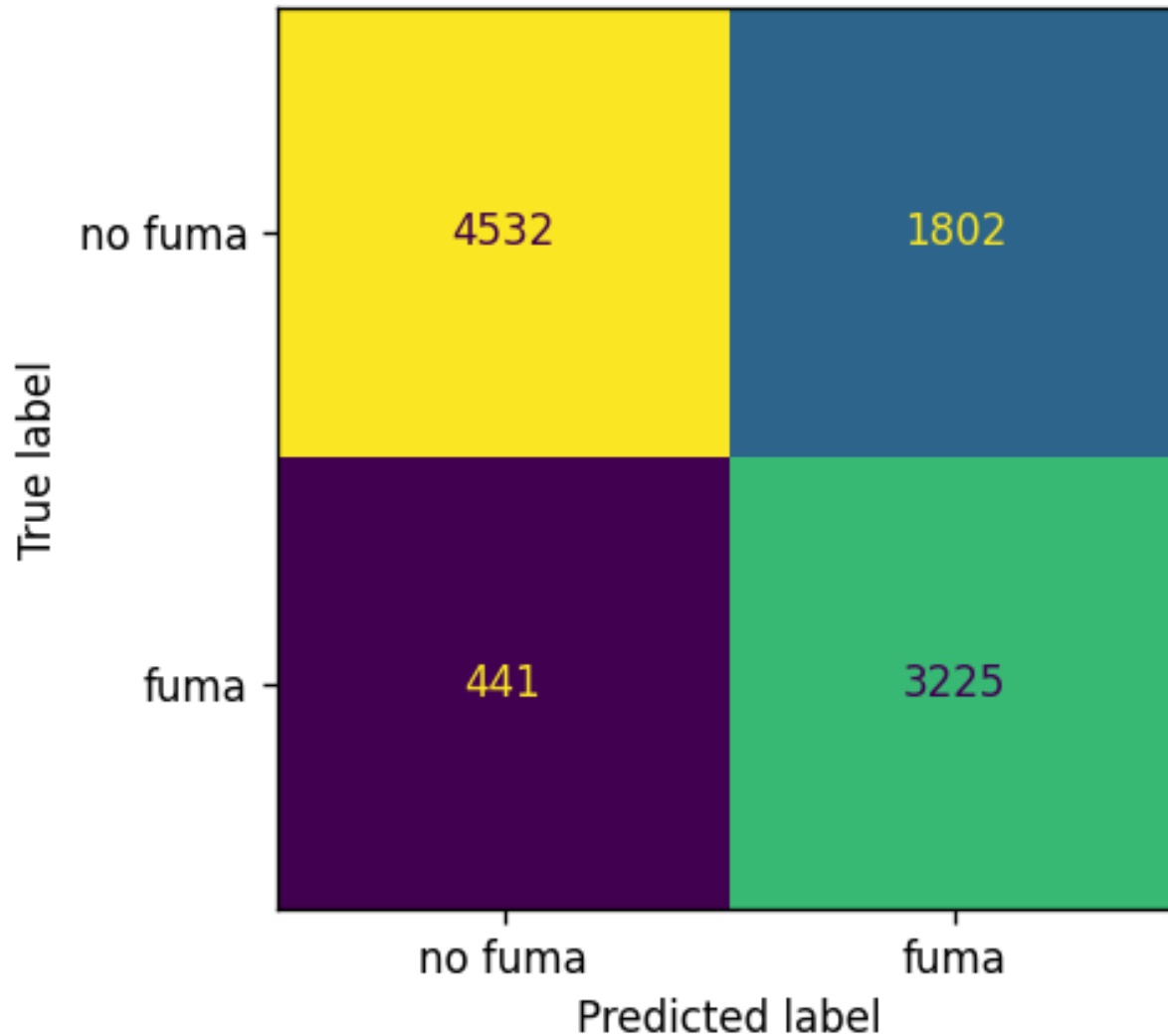
Matriz de confusion - XGBoost (thr=0.425)
