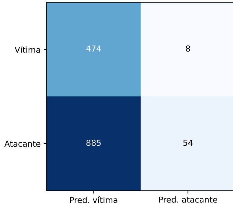
IF:c_completa — q990
