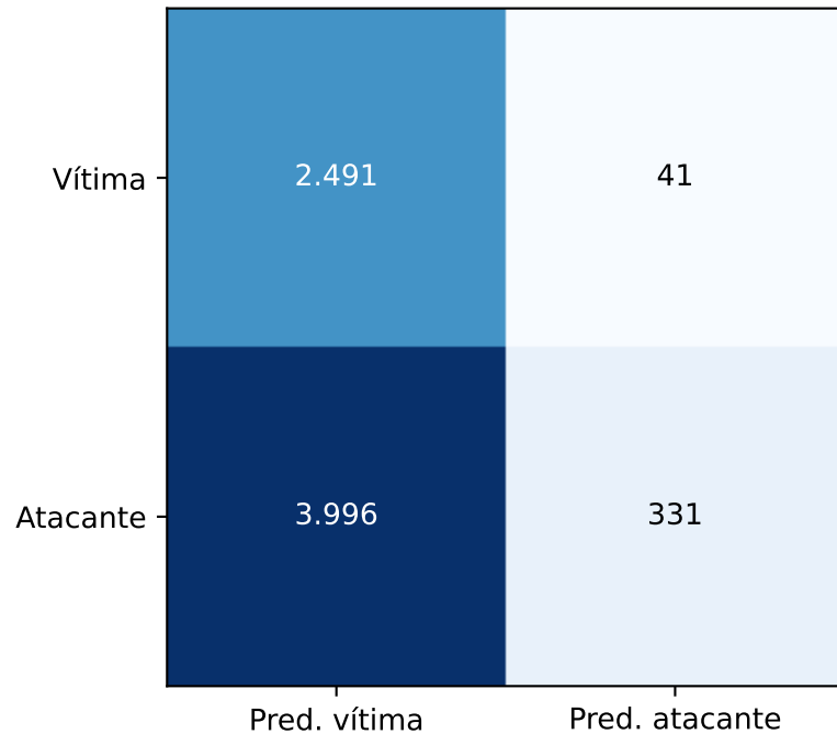
IF:b_completa — q990
