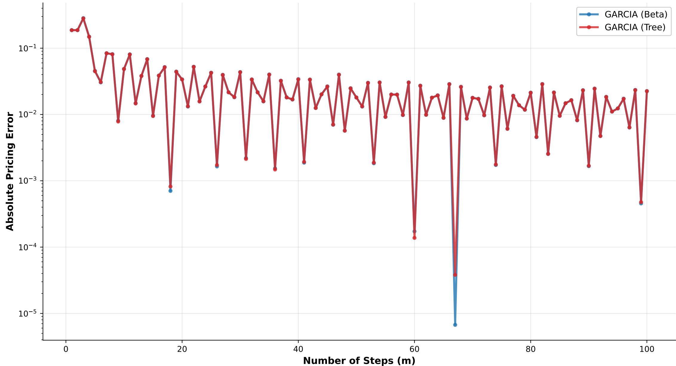
Digital Cash Call: Beta-Binomial vs Binomial Tree (Garcia)
