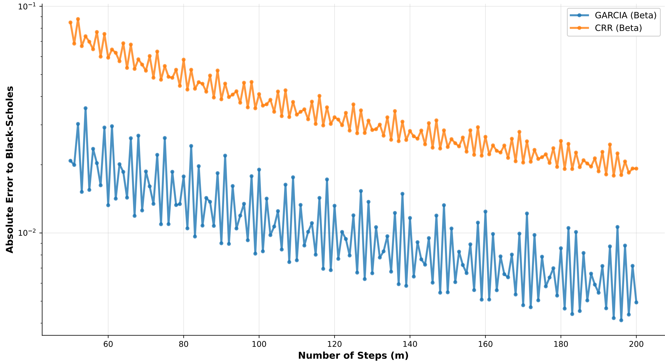
Vanilla Call: Garcia vs CRR Convergence
