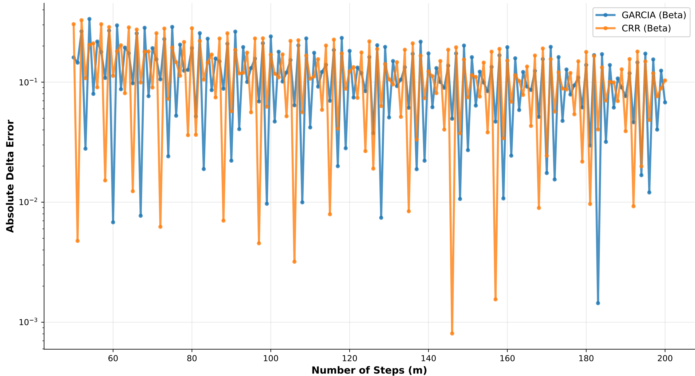
Digital Call Delta: Garcia vs CRR
