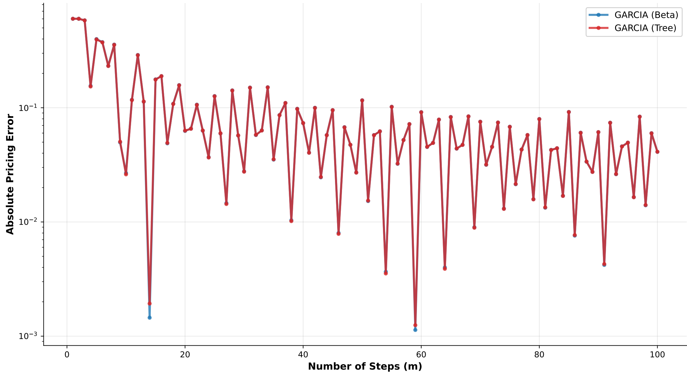
Barrier Call Up-Out: Beta-Binomial vs Binomial Tree (Garcia)
