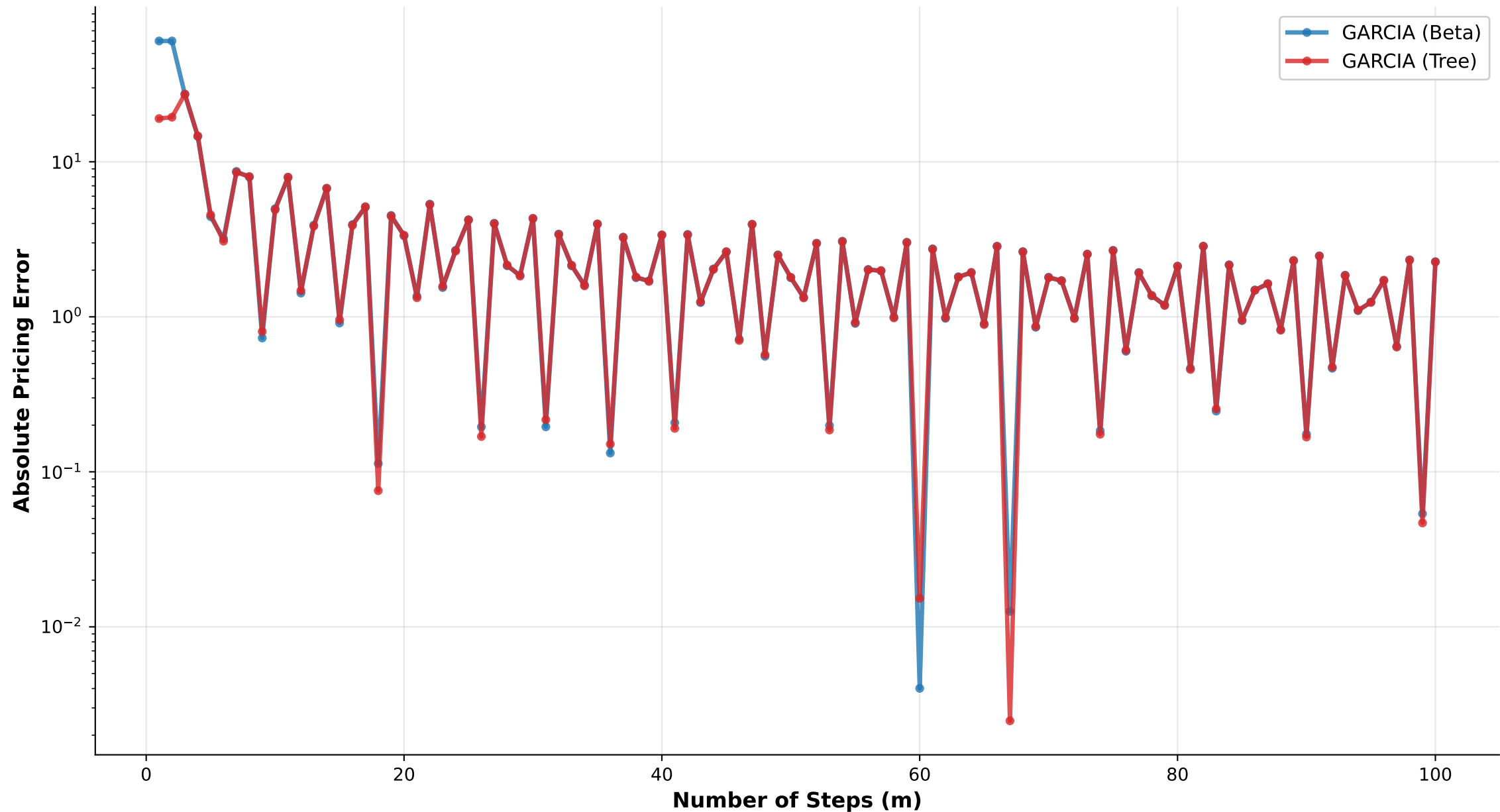
Digital Asset Put: Beta-Binomial vs Binomial Tree (Garcia)
