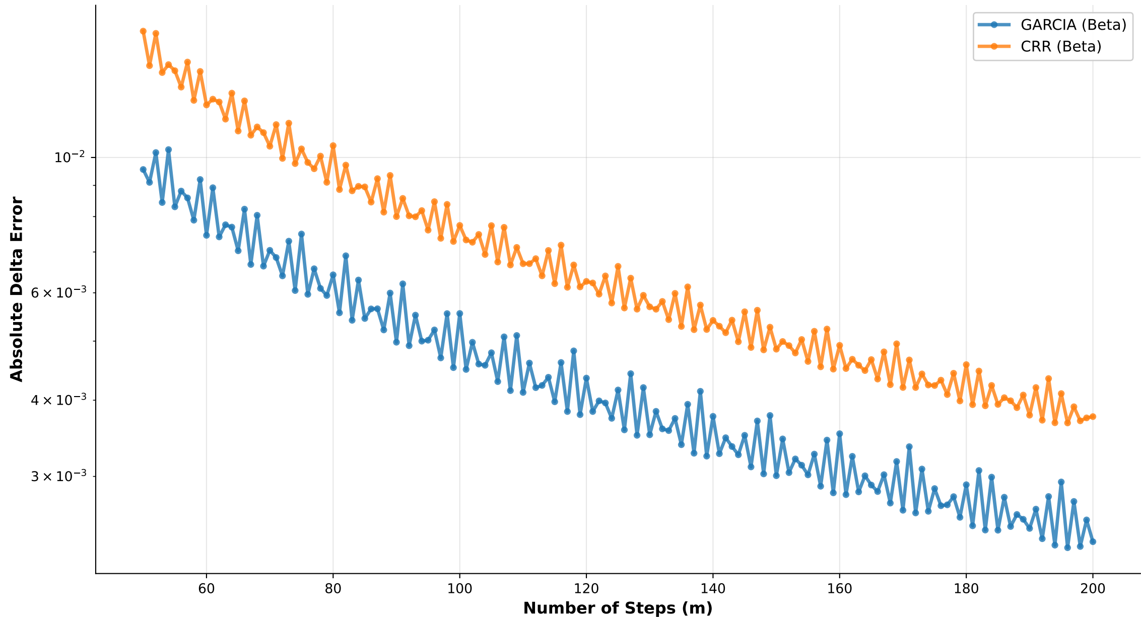
Vanilla Call Delta: Garcia vs CRR
