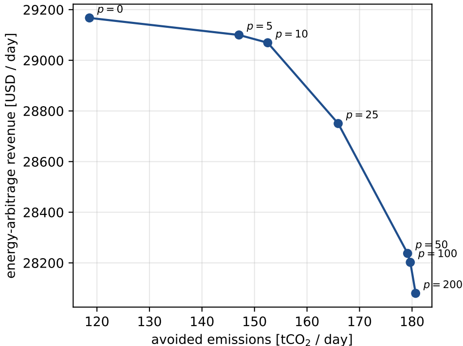
Revenue / abatement Pareto frontier -- BA S/E CRUCERO 220KV BP1
