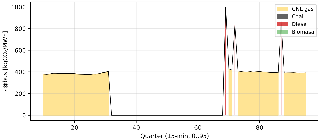
System-median marginal emission factor \varepsilon , 2026-04-22, by marginal fuel
