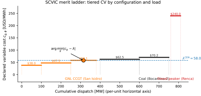
Fig. 3: SCVIC merit ladder for three illustrative units. The picker selects the tier whose CV is closest in absolute value to the target \lambda ; the highlighted marker shows the picked tier for \lambda = 58 \text{ USD MWh}^{-1} .
