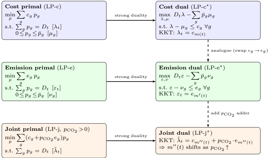
Fig. 4: Cost, emission, and joint primal/dual LPs. Strong duality and the swap c_g \leftrightarrow e_g produce the parallelism that justifies reconstructing \varepsilon_t from a published \lambda_t without resolving an LP.
