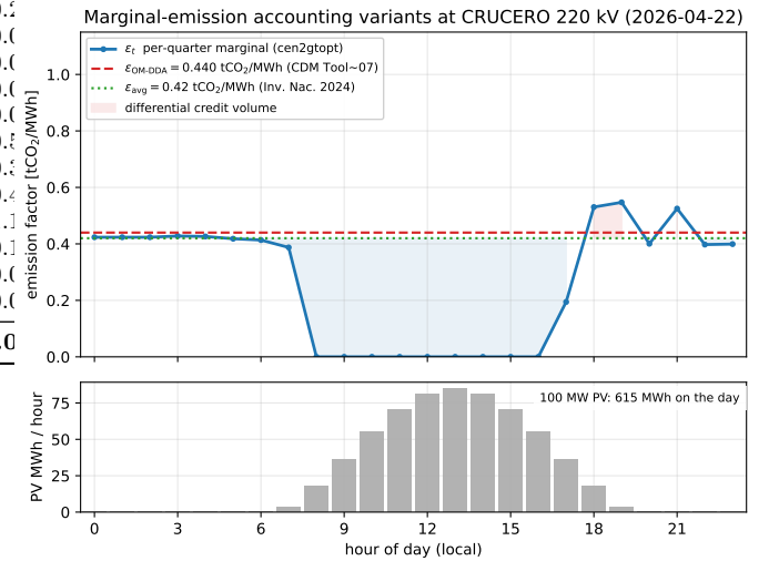
Fig. 11: 24-hour overlay at CRUCERO 220 kV on 2026-04-22: per-quarter \varepsilon_t from cen2gtopt (blue), dispatch-weighted OM-DDA per (23) (dashed red), and the 2024 Inventario Nacional national-average factor (dotted green). The shaded area between \varepsilon_t and \varepsilon_{avg} is the differential credit volume per accounting choice; the lower bar trace shows the hypothetical 100 MW PV plant’s hourly energy injection. Per-quarter values are taken from cen2gtopt ; the ten quarters without published \lambda^{CEN} are linearly interpolated.
