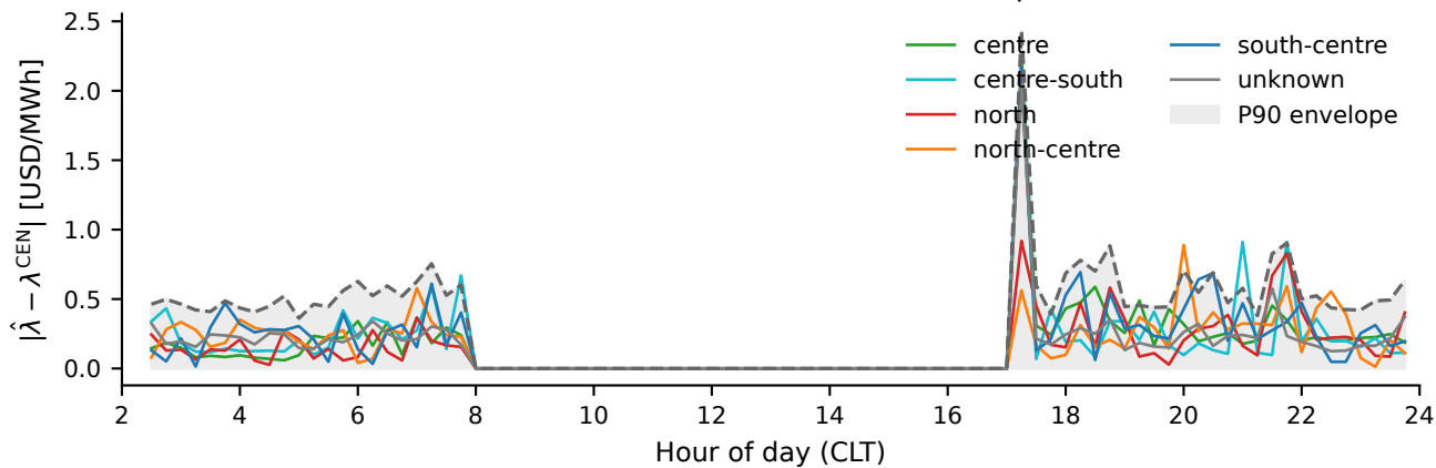
Panel C — Absolute reconstruction error per bus
