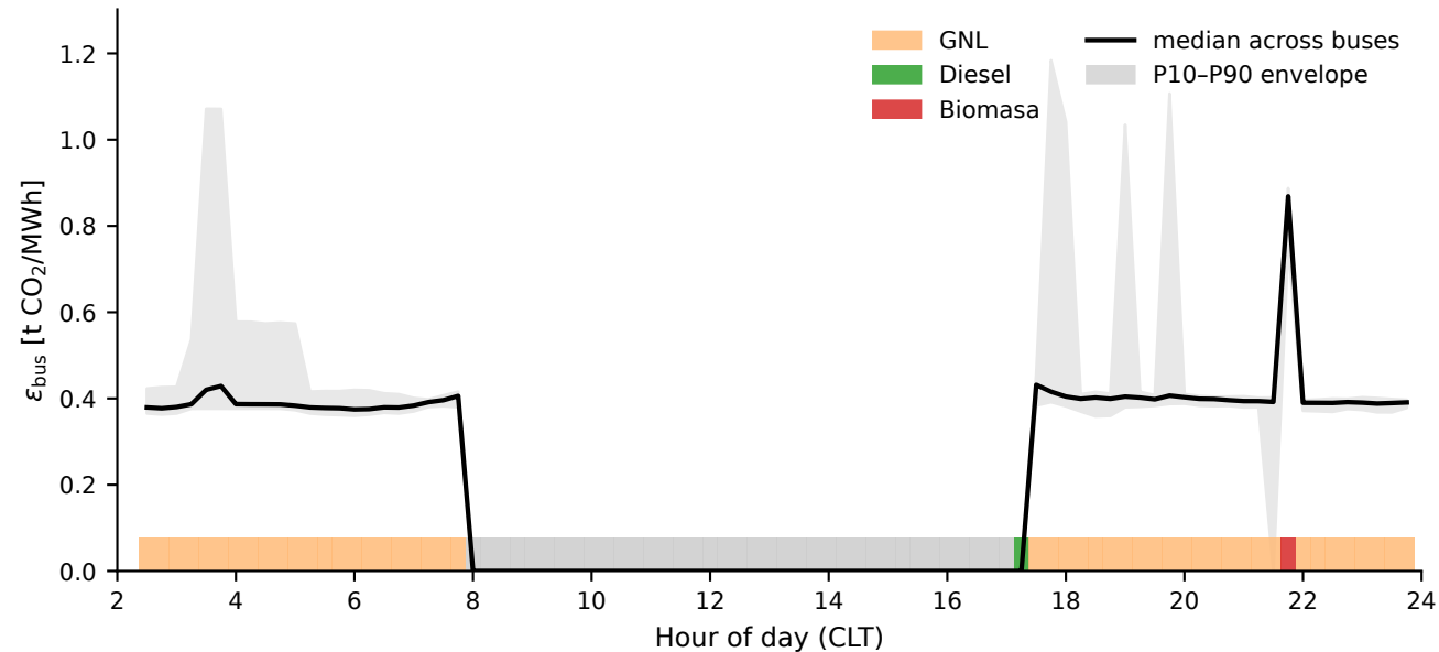
System marginal emission factor — 2026-04-22
