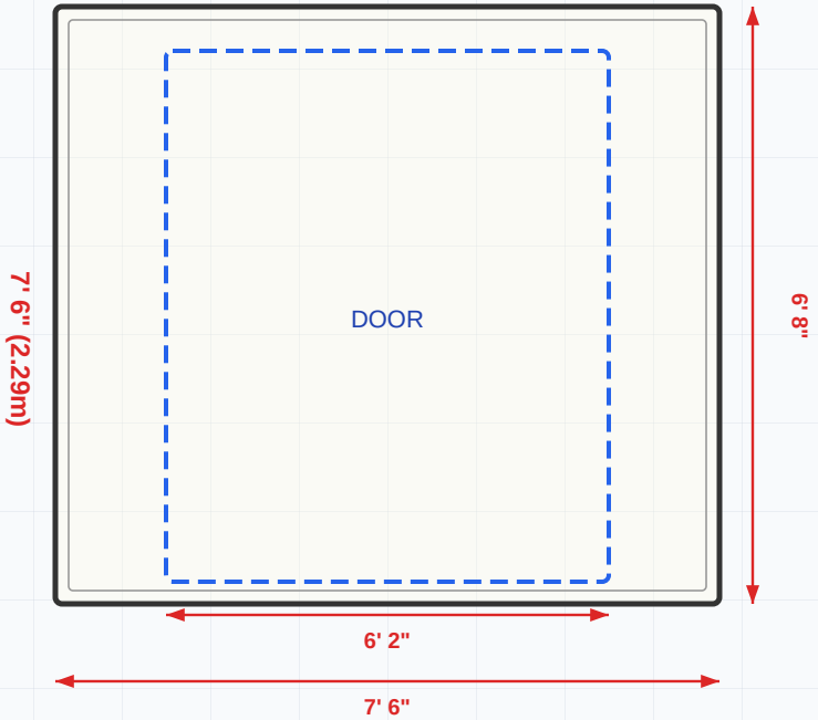
REAR VIEW (TRASERA)
