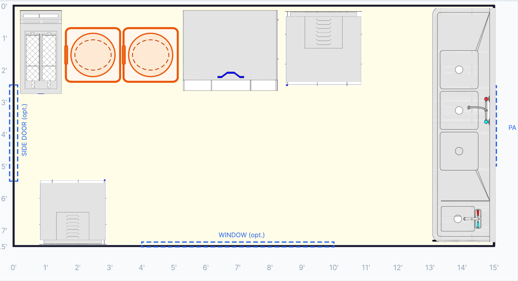
TOP VIEW (PLANTA)
