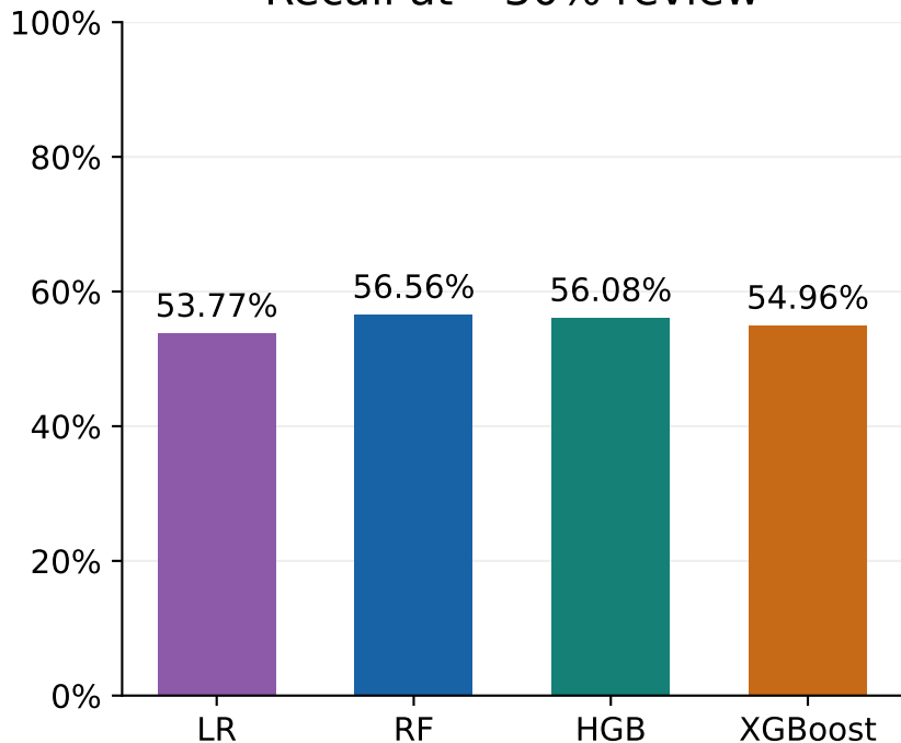
Recall at ~30% review
