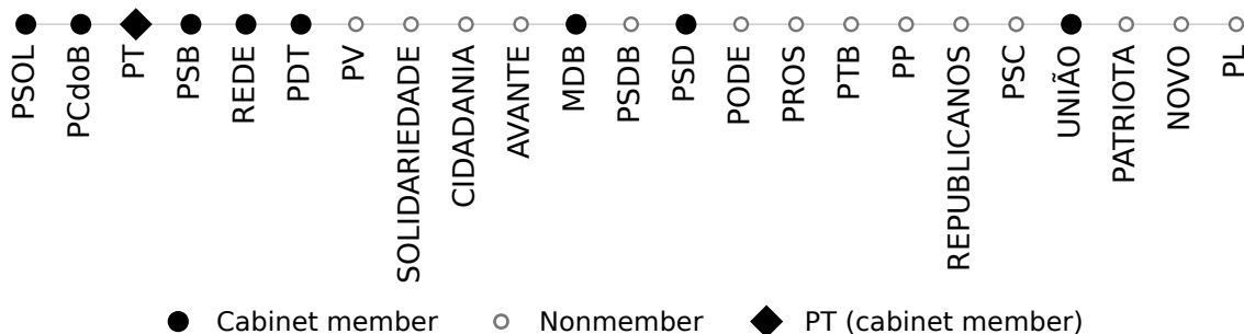
(b) Lula III | 2022 election | set 22-01 1 January-12 September 2023 | 48.89% votes, 263 seats
