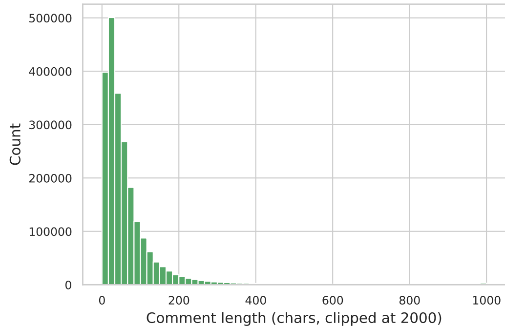
Comment length
