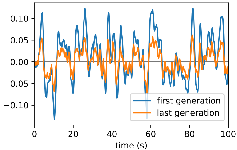
Particle position
