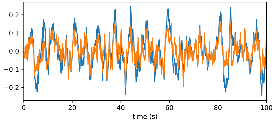
Particle velocity
