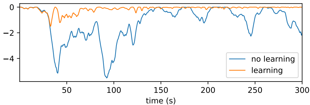
Instantaneous reward
