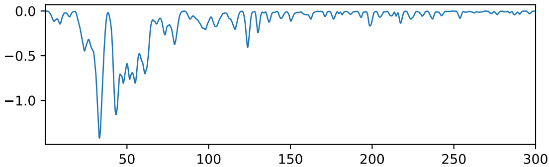
Estimated reward
