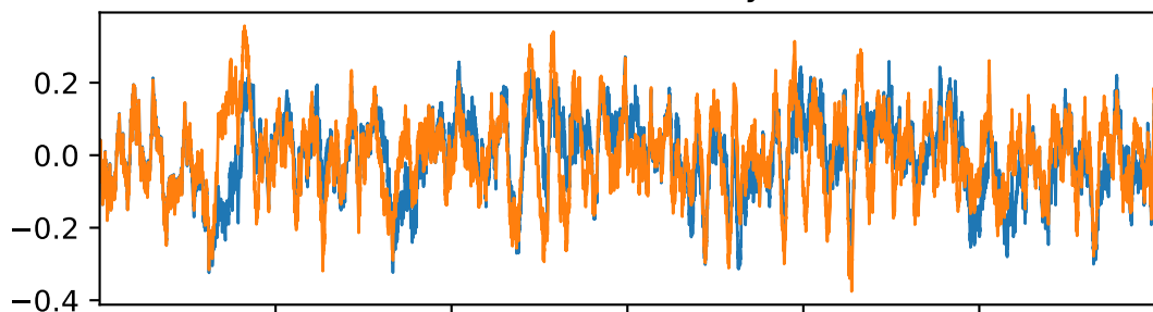
Instantaneous reward
