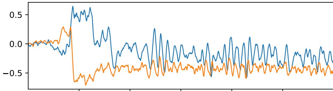
Neuron dynamics
