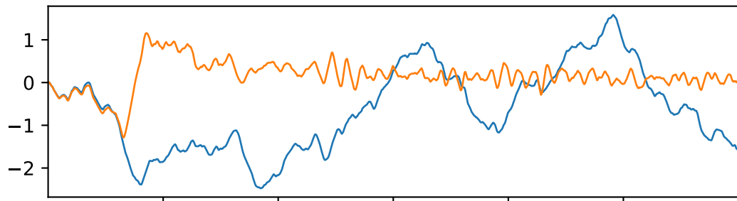
Particle velocity
