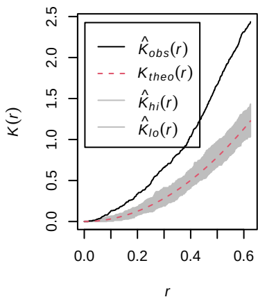
Reindeer
