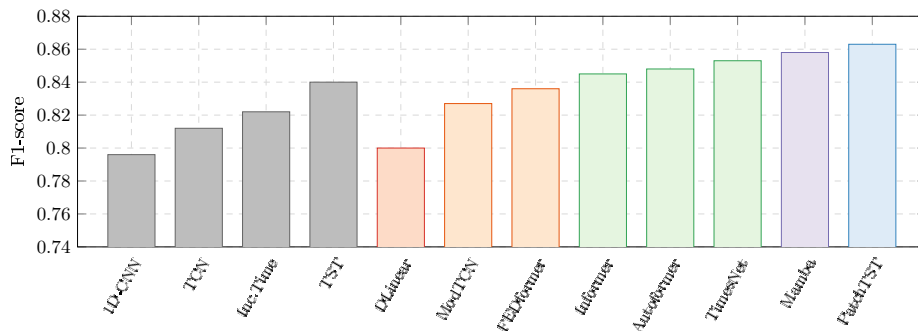
Fig. 3. Classification performance (F1-score) across all architectures under LOSO evaluation. Colour coding follows the computational complexity convention: grey = prior work [26], blue = O(N^2) patch attention, green = O(L \log L) (frequency/periodicity and sparse attention), purple = O(L) state space model, orange = O(L) (Fourier/convolution), red = O(L) linear baseline. The classical EDA feature-engineering baseline (F1 \approx 0.81, handcrafted SCR features + SVM) is reported in Table 3 and discussed in the text.
