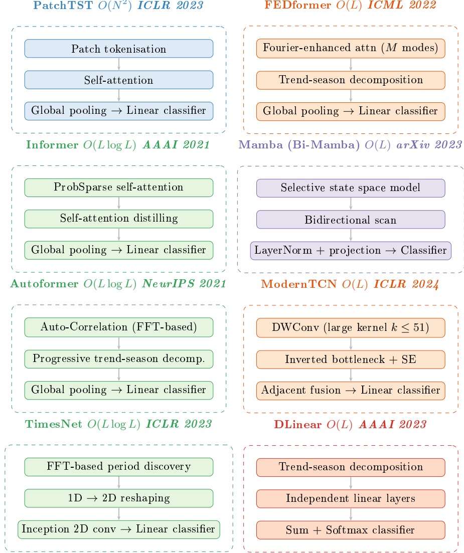
Fig. 2. Architectural overview of the eight models evaluated. Each architecture is organised as a three-stage pipeline (input transformation \rightarrow temporal modelling \rightarrow classification), grouped by paradigm family within dashed boundaries. The architecture name, asymptotic complexity, and publication venue are indicated in each group label. Table 1 provides a complementary summary. Colour coding follows the computational complexity class: blue = O(N^2) patch attention, green = O(L \log L) (frequency/periodicity and sparse attention), orange = O(L) (Fourier/convolution), purple = O(L) state space model, red = O(L) linear baseline.
