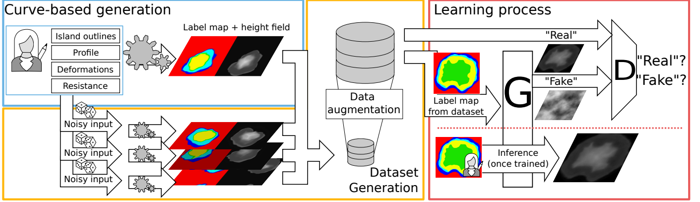
Figure 4: Blue box: our pipeline first prompts the user to create single pairs of coral reef island height fields and label maps using our proposed curve-based modelling algorithm (section 4). Yellow region: the same algorithm is applied multiple times on randomly altered versions of the user input to create a dataset, which we further enhance with data augmentation techniques (section 5). Redbox: finally, we train a conditional Generative Adversarial Network, which can then be used standalone to create height fields from labelled sketches (section 6).
