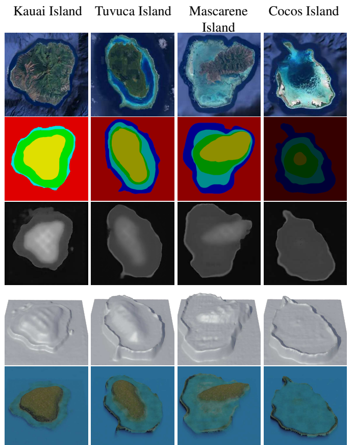
Figure 18: Reproduction of islands. From left to right: Kauai Island, Tuvuca Island, Mascarene Island, and Cocos Island.
