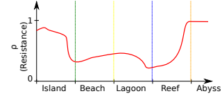
Figure 7: The resistance function of the island is defined with a similar strategy as the h_{\text{profile}} function. The resistance to erosion and deformation arises from multiple factors such as depth, materials, wind shadowing, biotic and abiotic factors, ... Modelling all these factors is complex. As such, using a user-defined approximation through a resistance function \rho allows for more control.
