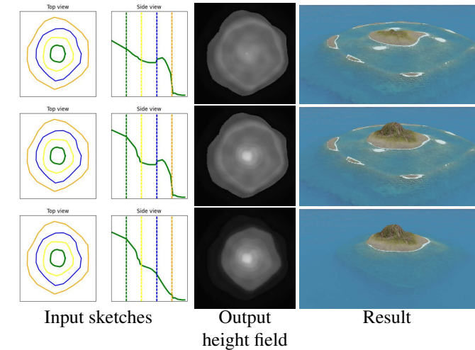
Figure 6: Providing a smooth function between each region results in islands with plausible reliefs. We fixed the outlines (first column) while editing only the height function (second column) in order to produce, from top to bottom, a low island, a coral reef island, and finally an identical island without the reef.
