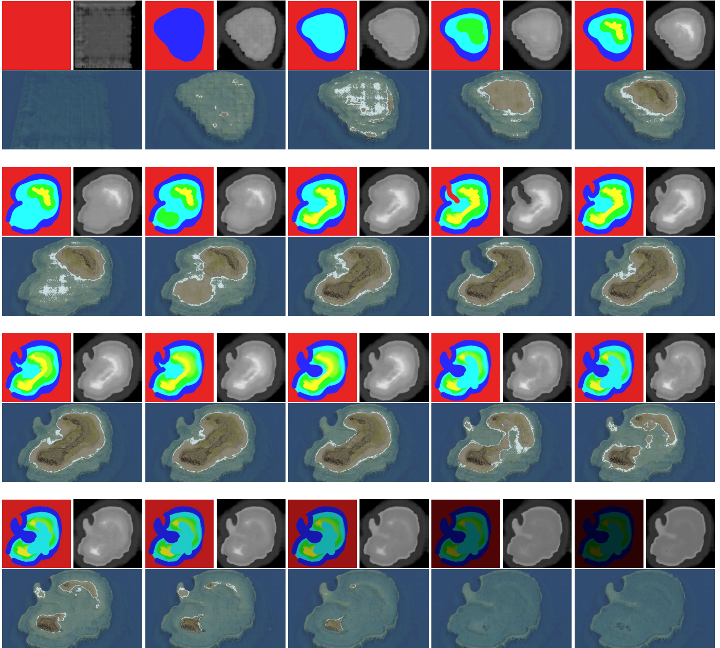
Figure 21: Few frames of an editing session for the generation of a coral reef island on Paint. The resulting height fields are output in real-time and each generation is consistent, allowing to interact fluently with the system without unexpected behaviour. The shaded outputs (bottom of each frame) are rendered in Blender, which are not real-time.
