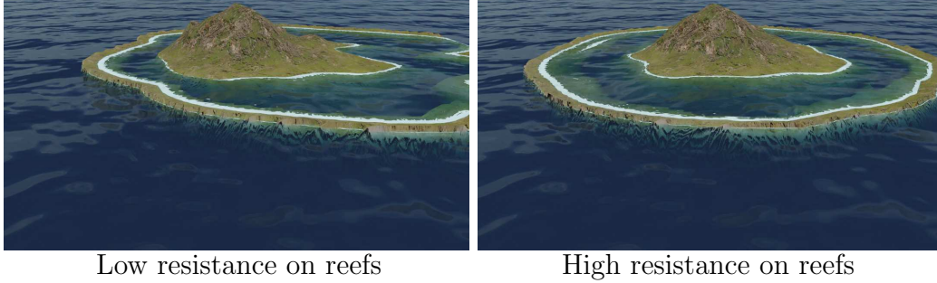
Figure 11: (Left) Given a uniform velocity field and a resistance function similar to fig. 12, the coasts are smoothly eroded while the interior of the island is almost unaffected. (Right) Modifying the resistance function to affect a strong resistance to borders emulates the effect of coast reinforcements.
