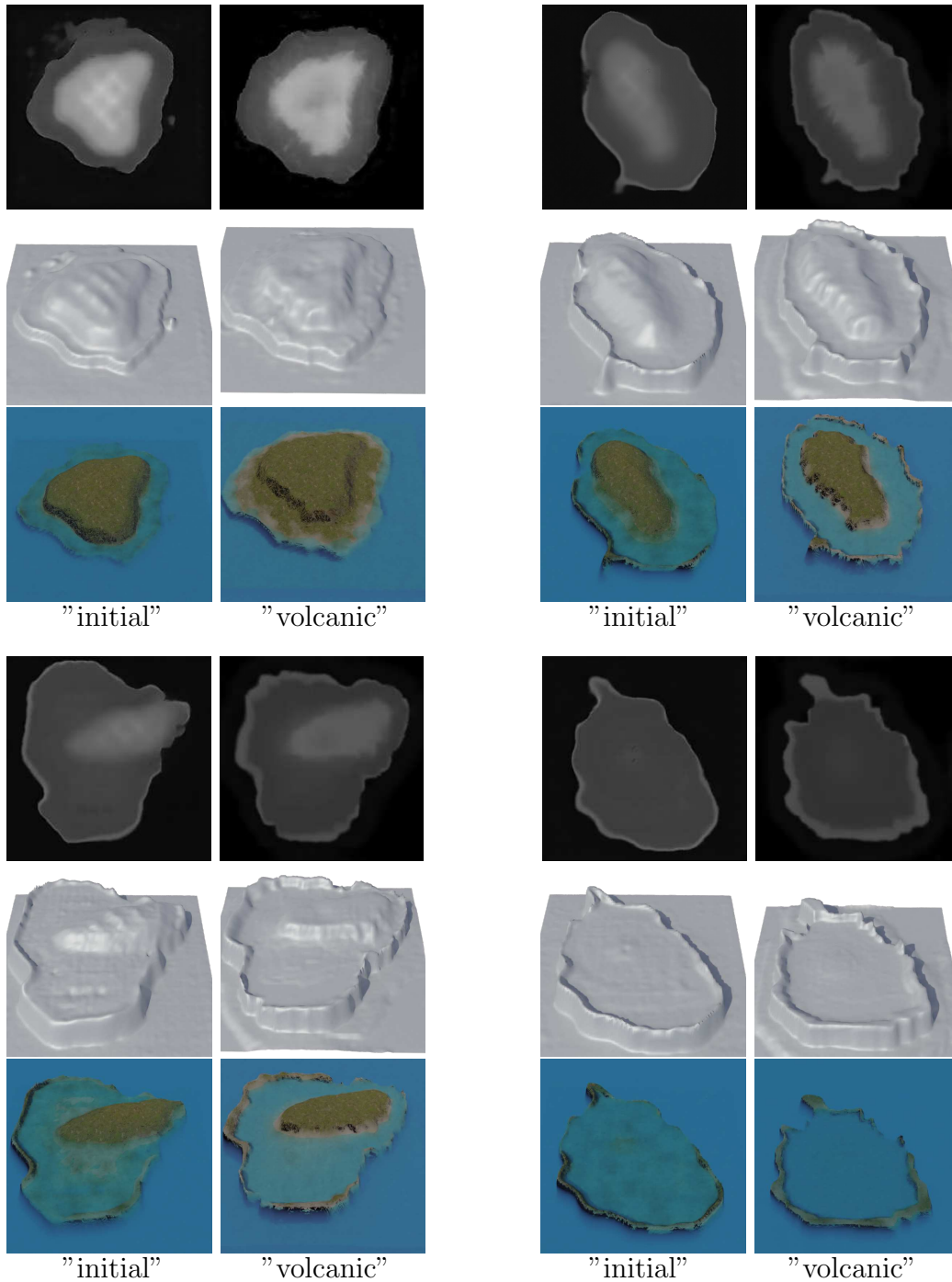
Figure 27: Comparison between the "initial" cGAN trained model (dataset generated from parameters visible in fig. 14) and the "volcanic" cGAN (fig. 27, top). The input label maps are identical as fig. 28.
