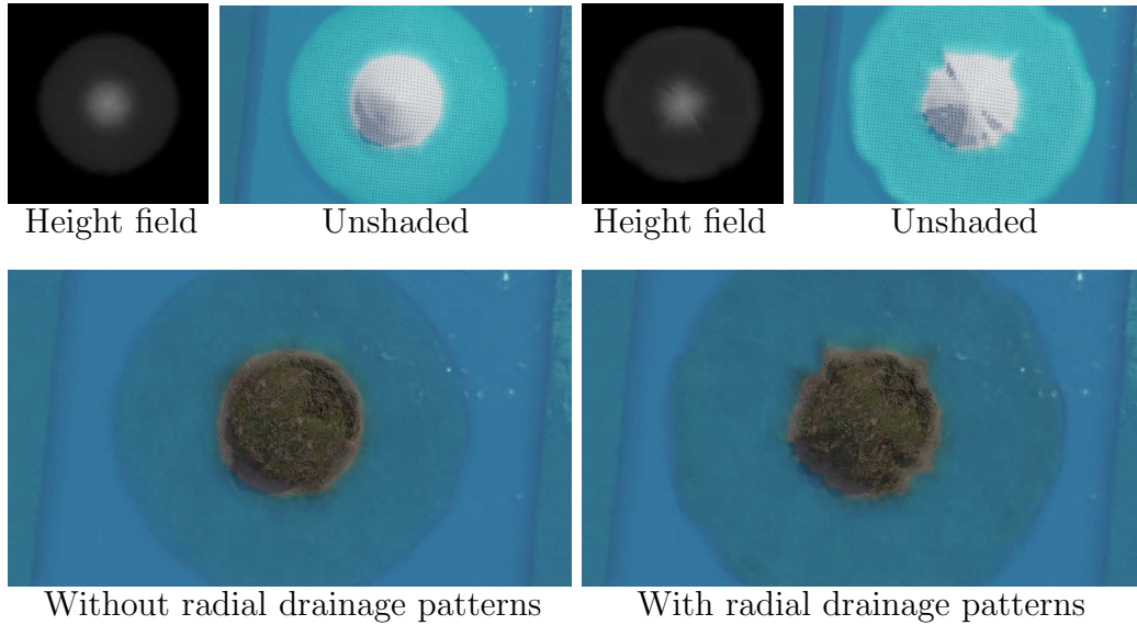
Figure 17: Multiple procedural strokes are added between the island centre and the surrounding sea, alternately landward and seaward. This transforms a simple circular island (left) into a more realistic volcanic island (right) by cheaply simulating star-shaped radial drainage patterns.
