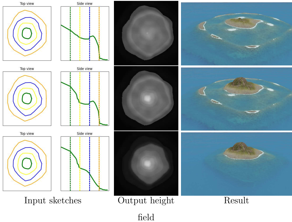
Figure 7: Providing a smooth function between each region results in islands with plausible reliefs. We fixed the outlines (first column) while editing only the height function (second column) in order to produce, from top to bottom, a low island, a coral reef island, and finally an identical island without the reef.
