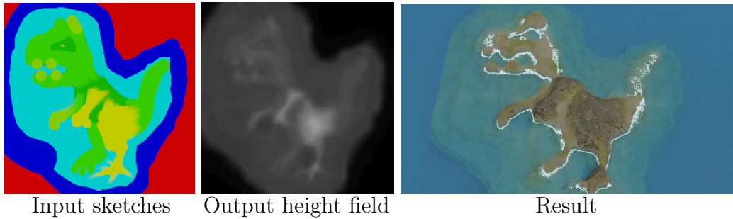
Figure 27: Without constraints on the generation, the user may use unrealistic layout and the neural network will however output a plausible result. Here new colours have been added (pistachio), but the network naturally considers it as a transition from mountain to beach.
