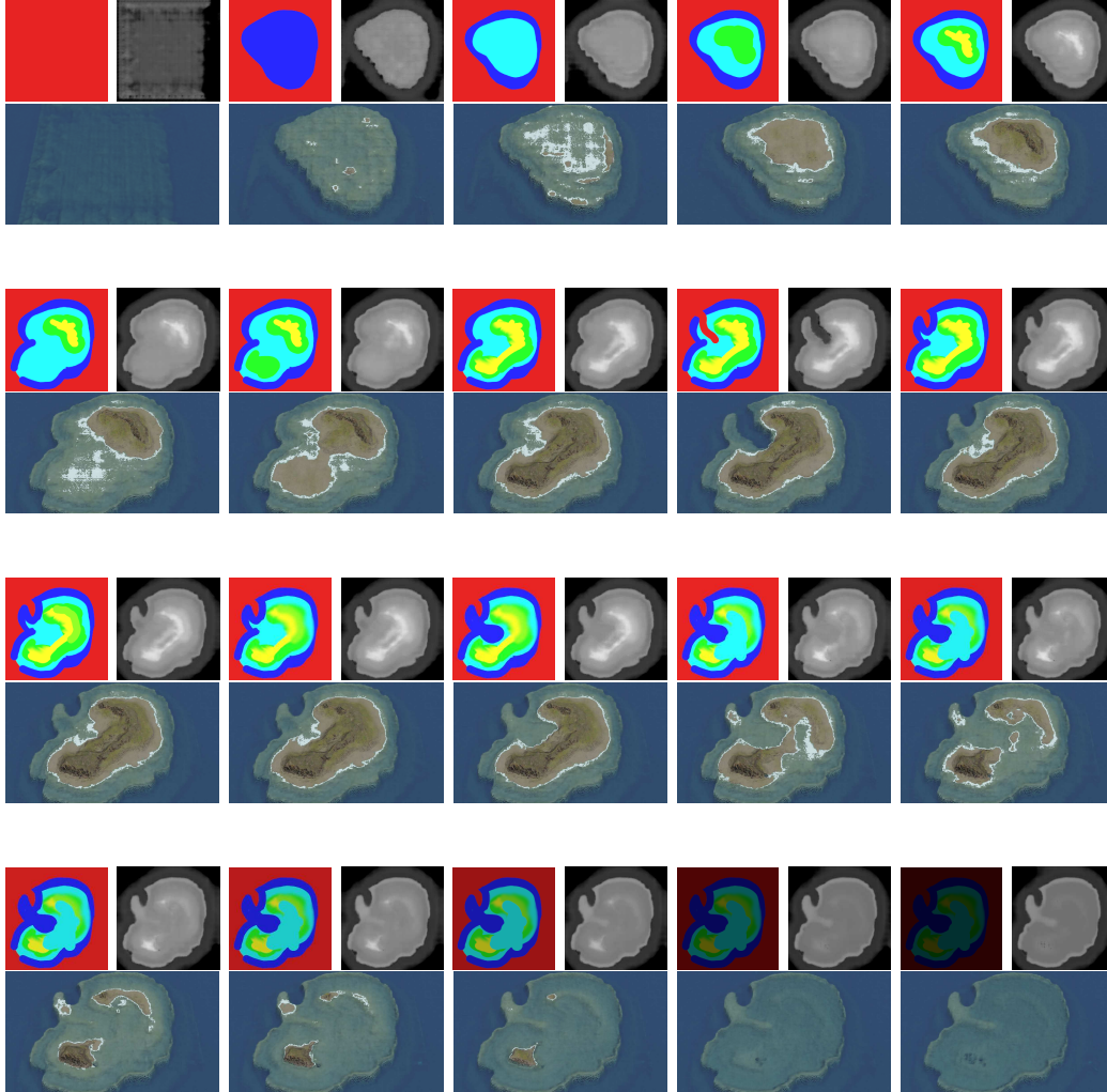
Figure 33: Few frames of an editing session for the generation of a coral reef island on Paint. The resulting height fields are output in real-time and each generation is consistent, allowing to interact fluently with the system without unexpected behaviour. The shaded outputs (bottom of each frame) are rendered in Blender, which are not real-time.
