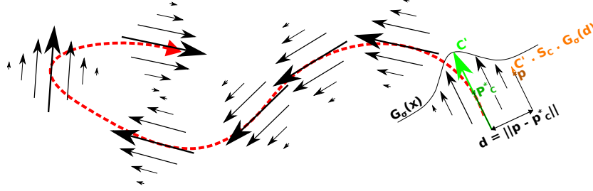
Figure 12: From the parametric curve defined by a user (red), we define the velocity field by considering the directional derivative C' of the curve C at the closest point \mathbf{p}_C^* , modulated by a Gaussian distance function G_\sigma(x) and scaled by the user-defined strength S_C .
