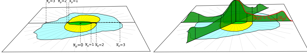
Figure 9: The \tilde{x}_{\mathbf{p}} parameter is used to stretch the 1D height function h_{\text{profile}}(x) to fit the distances from the centre to the outlines of each region defined in the top-view sketch.
