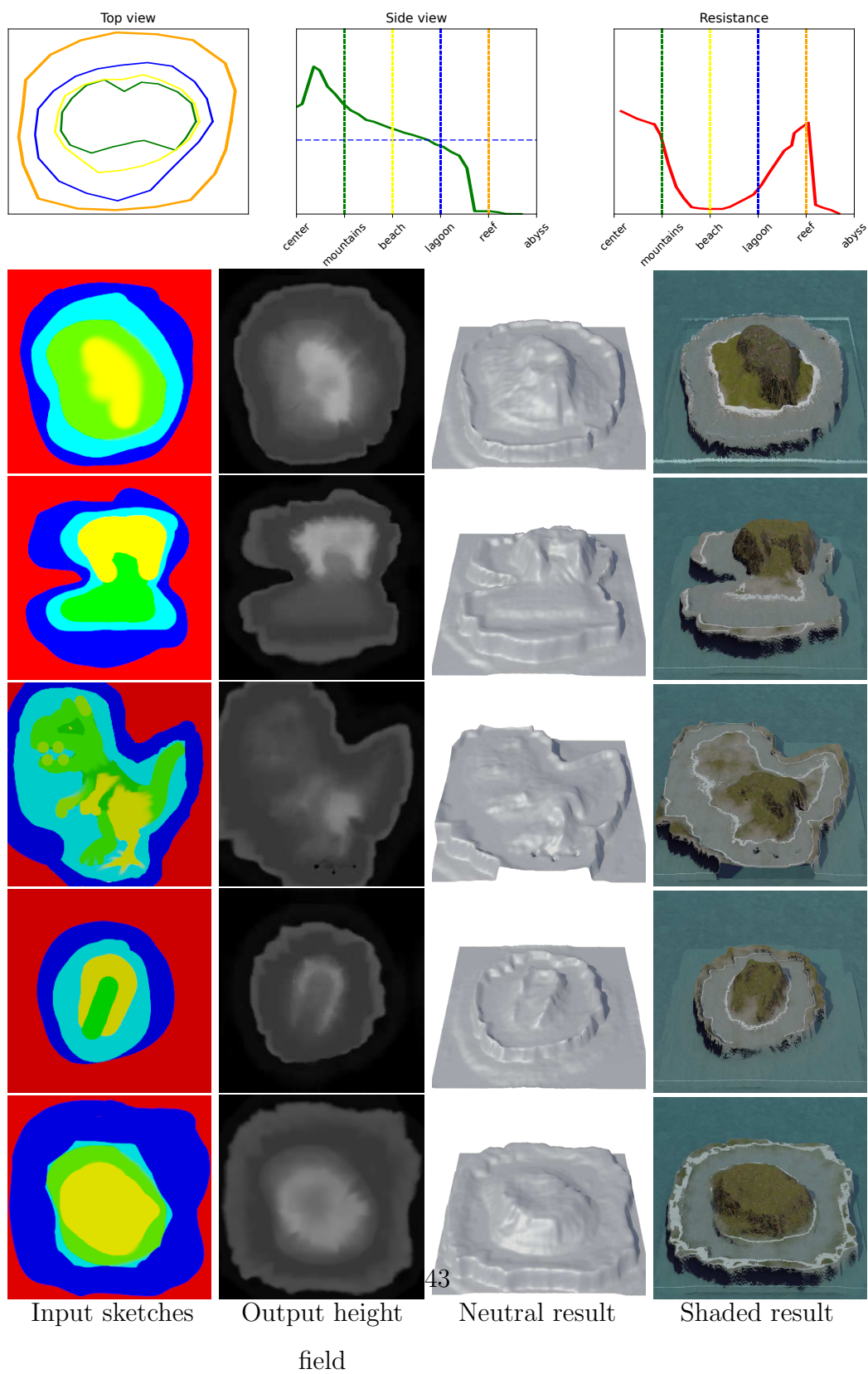
Figure 28: Top row: user input used to generate the "volcanic" dataset. Bottom: User sketches creates various islands, following the initial user inputs.
