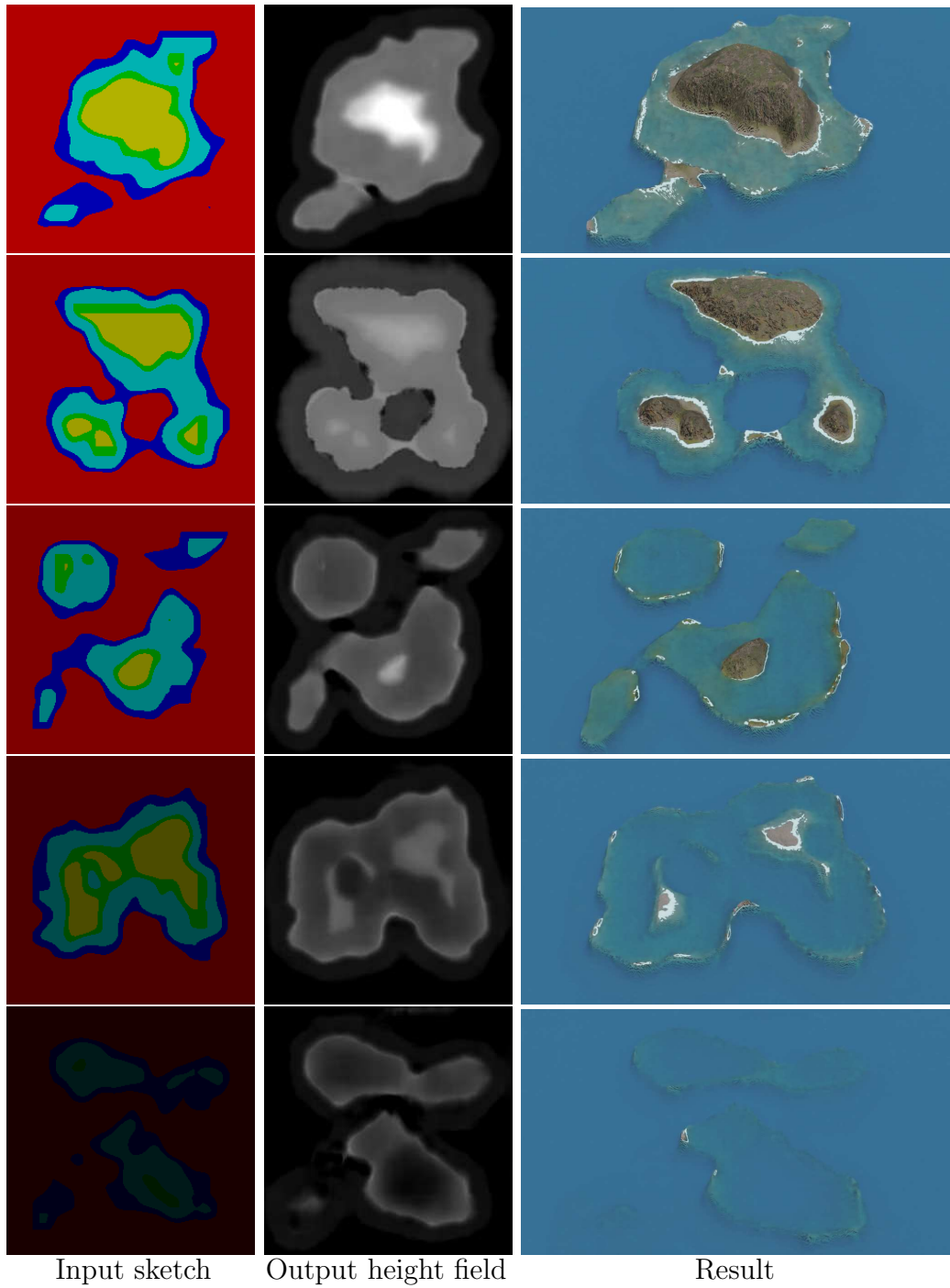
Figure 32: Starting from random Perlin noise, transformed into a label map, we can generate a large variety of results.
