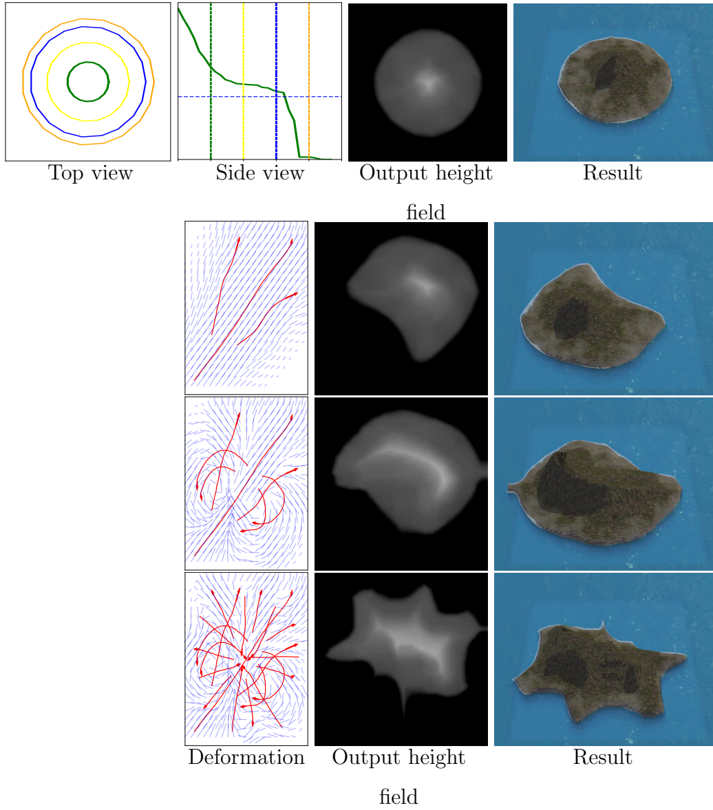
Figure 11: Top row: A circular island layout and a given profile sketch creates a simple round island height field. Each following row shows a progression in an edition session, conserving the initial top-view and side-view sketch, by manipulating the deformation field (blue lines) with respectively 3, 7 and 20 user strokes (red arrows). The final result breaks the initial radial symmetry of the island layout.
