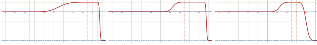
Figure 16: The modelling of the reef growth in our model is described by a piecewise function h_{\text{coral}} which is flat in the lagoon, the crest and abyss, and follows a smoothstep function as transitions for the back reef and fore reef regions. The model is easily edited by tuning the height values and delimitations of the subregions. Here, three examples of reef growth function with different delimitations (vertical dotted lines), providing more or less smooth transitions between reef subregions.
