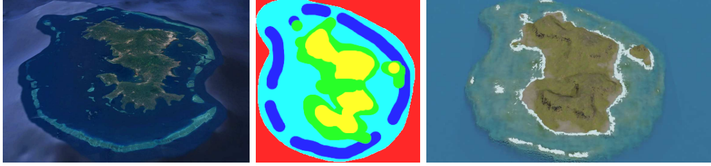
Figure 31: Comparison between real (left, from Google Earth) and synthetic (right) islands of Mayotte. The label map (centre) is hand-drawn to match approximately its real-world counterpart.
