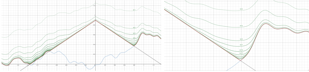
Figure 18: Blending two functions f : \mathbb{R} \mapsto \mathbb{R} (black, dotted) and g : \mathbb{R} \mapsto \mathbb{R} (blue, dotted) with the max operator (red curve), causing discontinuities when f(x) = g(x) , and with the \text{smax} operator (green curves) with various sharpness values k , resolving the issue at the cost of slight overestimations with low values of k . Right presents a zoom on the domain x \in [0.5, 1.3] .
