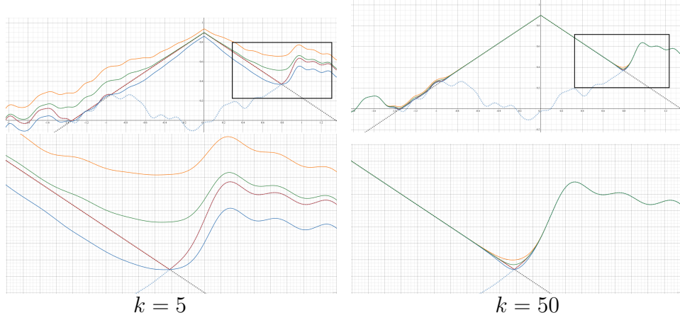
Figure 17: The \text{smax}^+ operator (orange curve) is a function that is used to overestimate the maximum value of two input functions (dotted curves), especially when the difference between the two functions is small, while the \text{smax}^- function (blue curve) tends to underestimate the max operator. Taking \text{smax} (green curve) as the average of \text{smax}^- and \text{smax}^+ creates a smooth function closely approximating the max operator, even with low values of sharpness k (Left: k = 5 , right: k = 50 ). Bottom graphs show a zoom on the domain x \in [0.5, 1.3] .
