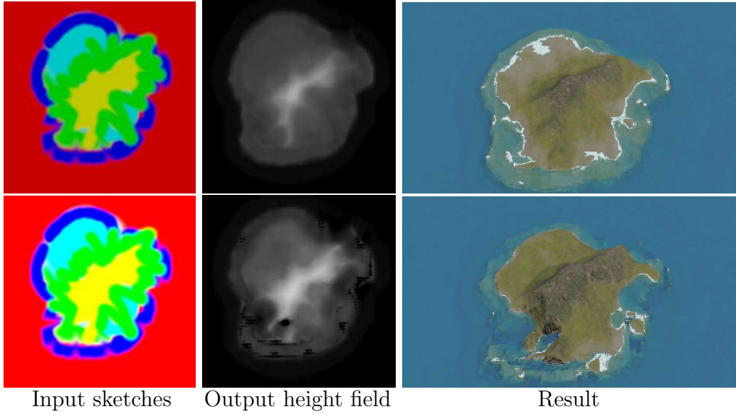
Figure 26: User applied fuzzy brushes to draw the label map, resulting in some pixels that are inconsistent with the dataset and illogical island layouts: abyss regions (red) are found between beach (green), lagoon (cyan) and reef regions (blue). The neural model ignores the layout inconsistencies, and partial over-brightness as long as the pixel is not completely white.
