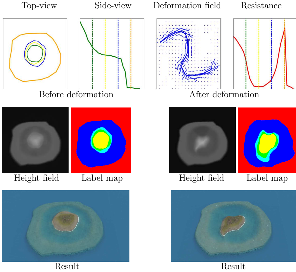
Figure 15: A top-view velocity field is defined from user-provided strokes (top, blue), in association with a resistance function (top, red); a height field is deformed accordingly. Left: original height field and render; right: altered results. The beach and lagoon regions are defined with low resistance, which is visible by having only these regions deformed in bottom results.
