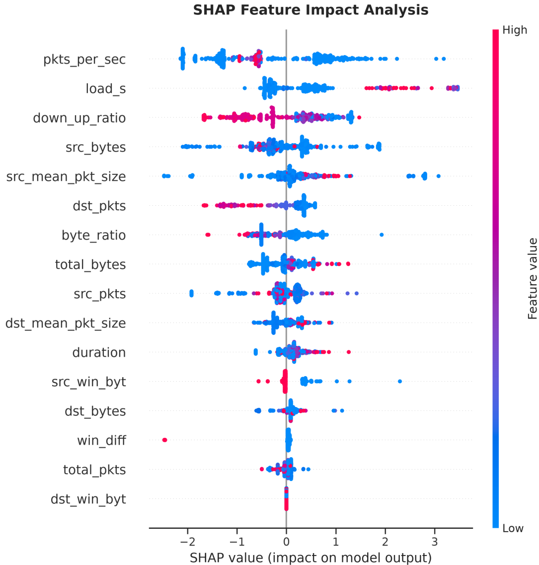
Figura 5.8: Summary plot SHAP della baseline INJ. implementata mediante Histogram-based Gradient Boosting, valutata sul test set INJECTION con seed s = 42 .
