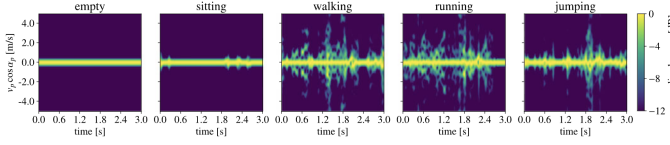
Fig. 3: Doppler spectrograms for different cases [1]
