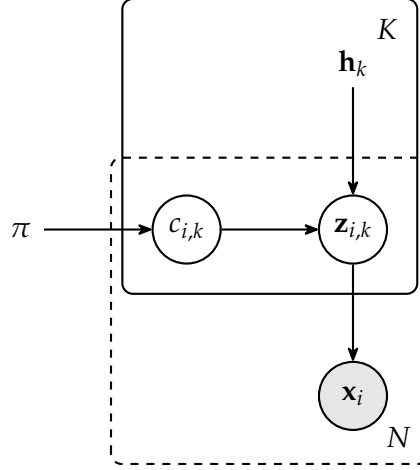
Figure 3.1: The VAAE generative model as a probabilistic graphical model. For each of the K concepts, a binary mask c_{i,k} (drawn from a Bernoulli with rate \pi ) gates a Gaussian embedding \mathbf{z}_{i,k} centred either at the origin or at the learned prototype \mathbf{h}_k ; the gated embeddings generate the observation \mathbf{x}_i . Shaded nodes are observed and unshaded latent, bare symbols are global parameters; the solid plate replicates over concepts and the dashed plate over the N observations.
