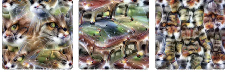
Figure 2.3: Neuron 4e:55, a polysemantic neuron from InceptionV1 which responds to cat faces, fronts of cars, and cat legs. Reproduced from Olah et al. [25].
