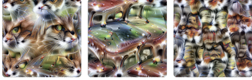
Figure 2.3: Neuron 4e:55, a polysemantic neuron from InceptionV1 which responds to cat faces, fronts of cars, and cat legs. Reproduced from Olah et al. [27].
