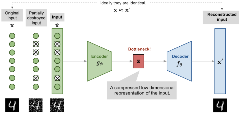
Figure 2.2: Illustration of Denoising autoencoder model architecture, reproduced from Weng [51]. Note: this figure uses f for the decoder and g for the encoder, the reverse of the letter convention adopted in this thesis.
