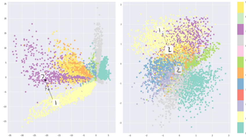
Figure 2.3: Two-dimensional latent spaces learned on MNIST, coloured by digit class, reproduced from Shafkat [41]. Optimising for reconstruction alone (left) lets a standard autoencoder separate the classes into disconnected clusters with gaps that decode to unrealistic samples, whereas the Variational AutoEncoder objective (right) yields a smoother, more continuous arrangement, concentrated around the origin by the prior, that can be sampled and interpolated.
