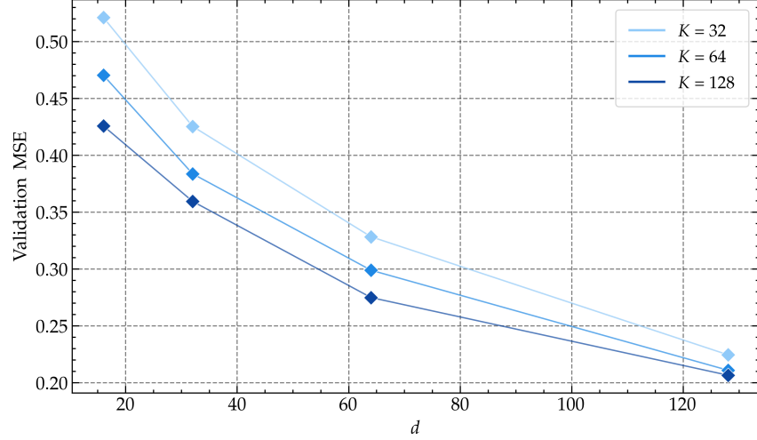
Figure 4.4: Effect of the per-concept embedding width d on VAE reconstruction. Validation MSE against d \in \{16, 32, 64, 128\} , one curve per dictionary size K \in \{32, 64, 128\} , all at the fixed sparsity target \tilde{\kappa} = \pi K = 8 , so that only the embedding width varies along each curve. Reconstruction improves with d , with diminishing returns — widening a concept adds capacity that a scalar atom cannot, though at the cost of more active neurons ( \ell_0 = \kappa d ) and more parameters.
